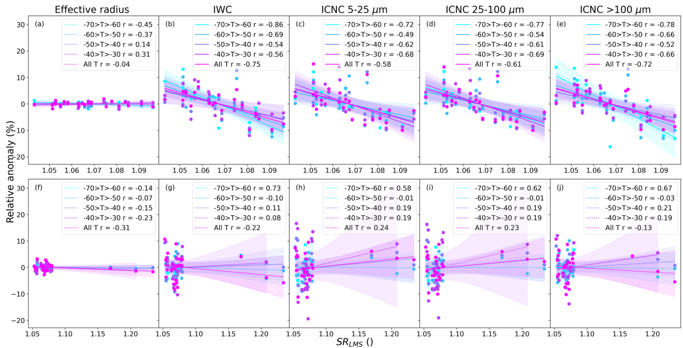
Figure 2. Monthly averaged DARDAR data of microphysical properties of cirrus clouds at different temperatures plotted against the aerosol scattering ratio in the LMS ( SR_{LMS} ). The DARDAR data are the relative anomaly from a long-term average for each month (see Section Text S2 in Supporting Information S1). The results from the NH ( 40^{\circ} – 60^{\circ} ) are shown on the top row and the results from the SH ( -60^{\circ} to -40^{\circ} ) on the bottom row. The lines show linear regressions and solid lines indicate a statistically significant correlation between the two variables ( p -value < 0.05 ) and the shaded areas show the 95% confidence intervals for the predicted values. The correlation coefficients between the variables are shown in the legend. Note the different scales on the x axis for the NH and SH.
