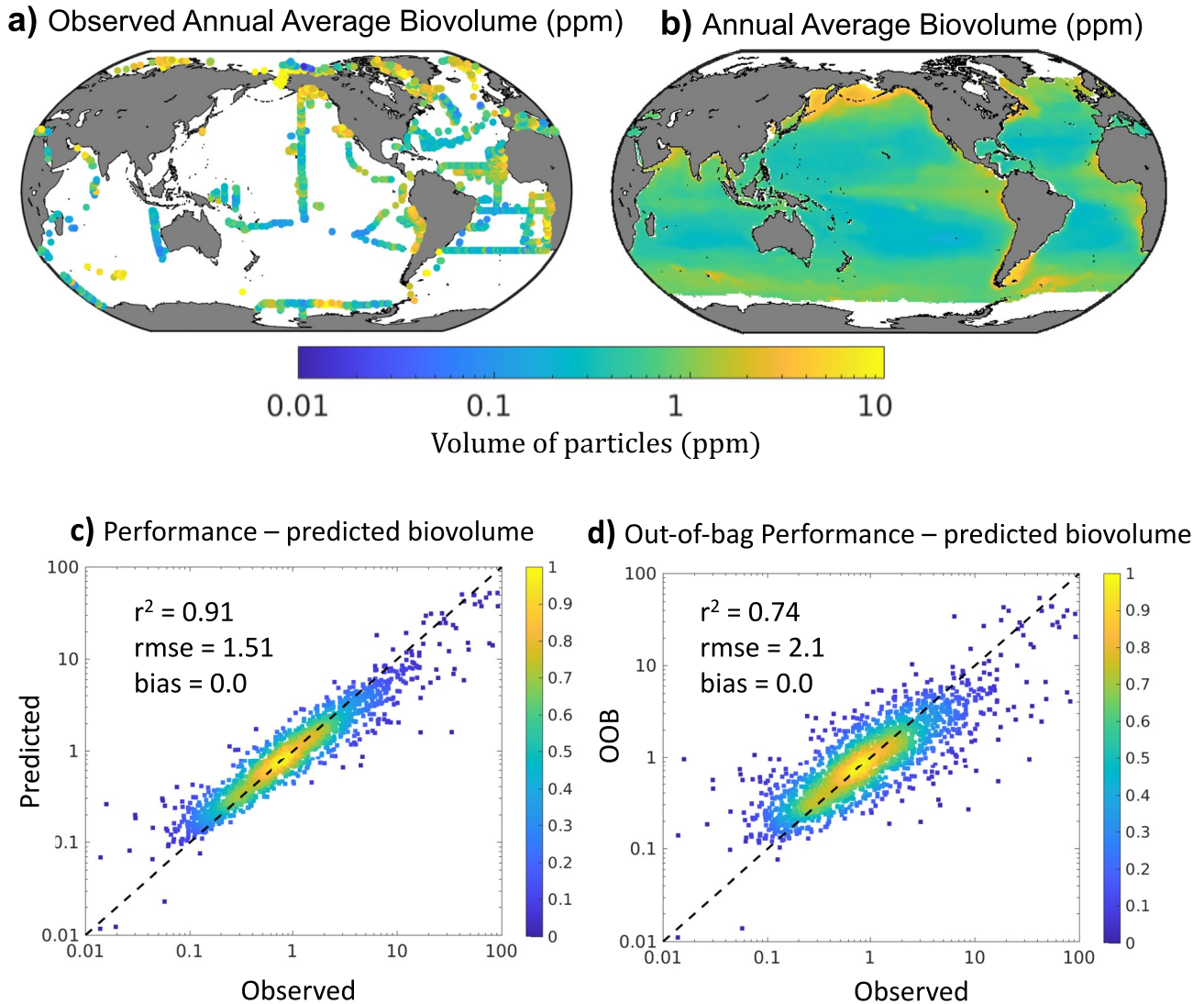
Figure 3. Observed and reconstructed particle biovolume (BV, in parts per million, ppm) at the base of the euphotic zone. (a) Observed average BV. (b) Annual mean BV reconstructions. (c) Performance of the Random Forest reconstruction shown as density scatter plots of predicted versus observed BV (colors indicate the normalized density of observations at each point). Panel (d) same as panel (c), but using out-of-bag (OOB) predictions, that is, predictions versus observations withheld from training. Annotations in panels (b and c) show the coefficient of determination ( r^2 ), the RMSE, and the global bias.
