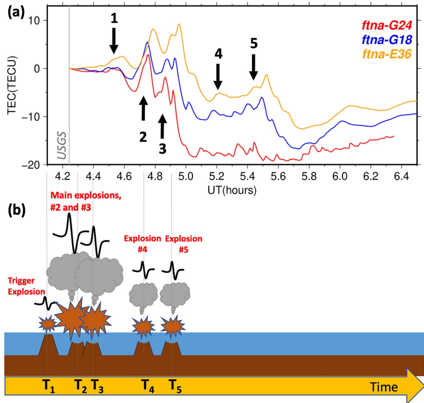
Figure 2. (a) Ionospheric disturbances corresponding to five explosions that most likely took place on 15 January 2022. Gray vertical line denotes the US Geological Survey onset time; (b) Suggested scenario and the timeline of the HTHH volcano explosions of 15 January 2022. Each explosion emits an acoustic pulse of different amplitude as illustrated. Vertical dotted lines correspond to the ionospherically determined onset times of the explosions.
