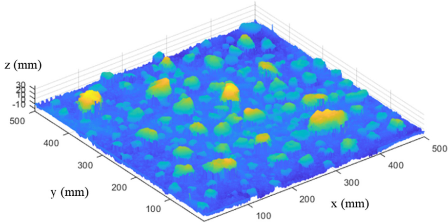
Fig. 2 – 2.5D DEM of second laboratory soil surface with high clod concentration at initial stage.
