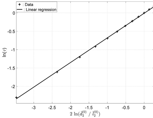
Fig. 5 – Data points (2 \ln(\bar{d}_2^{(0)}(\tau) / \bar{l}_2^{(0)}); \ln(\tau)) and linear regression for determination of roughness exponent for the second laboratory surface at initial state.
