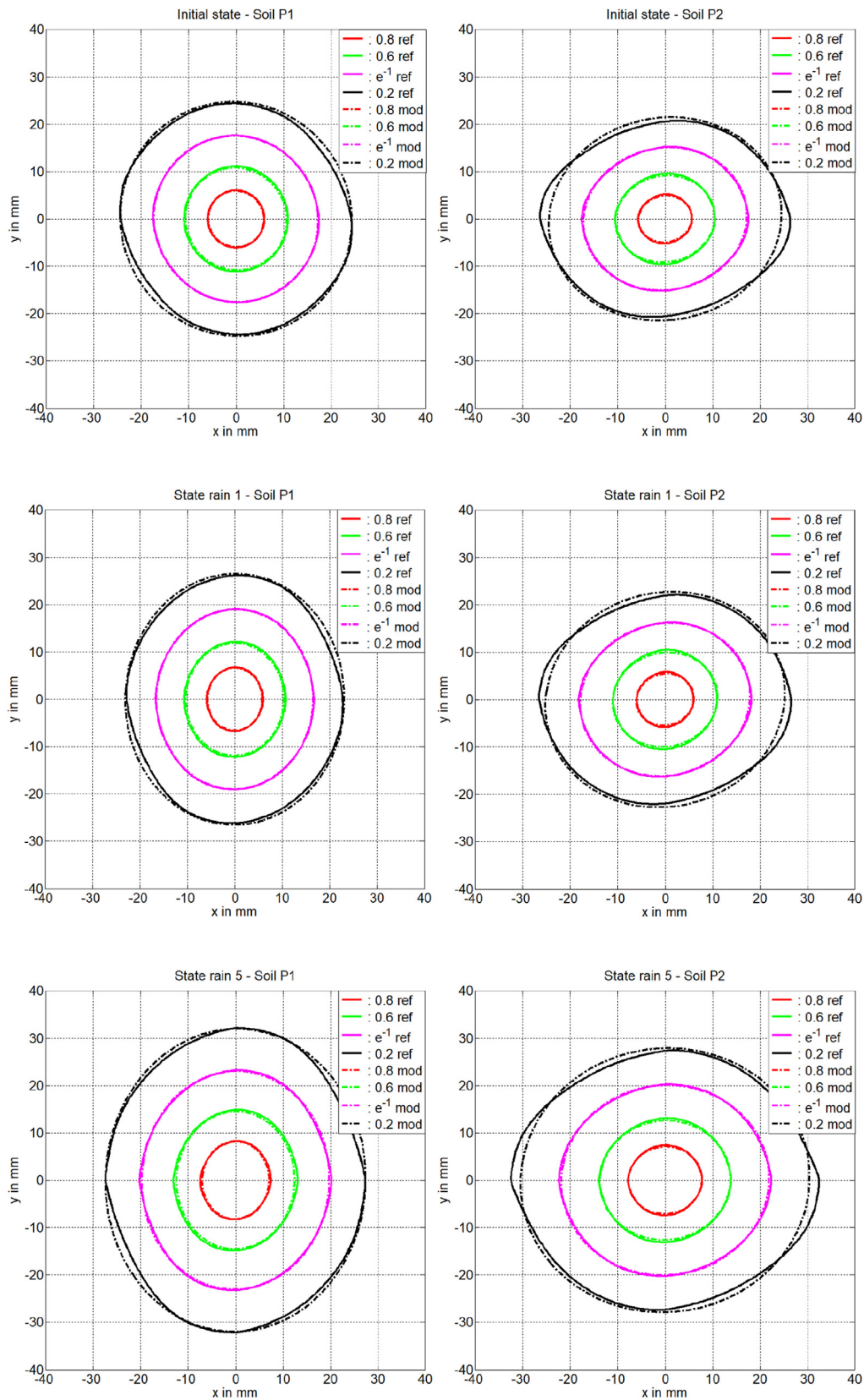
Fig. 6 – Level curves of reference autocorrelation function and modelled function for four values of the height expressed as a percentage of the variance. Laboratory made soil surfaces with a low clod concentration (left column), with a high clod concentration (right column).
