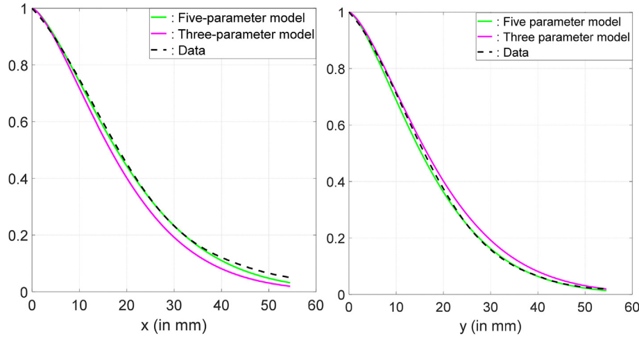
Fig. 4 – Normalised autocorrelation functions with respect to Ox axis (left column) and Oy axis. (right column) for the first laboratory soil surface at final state.
