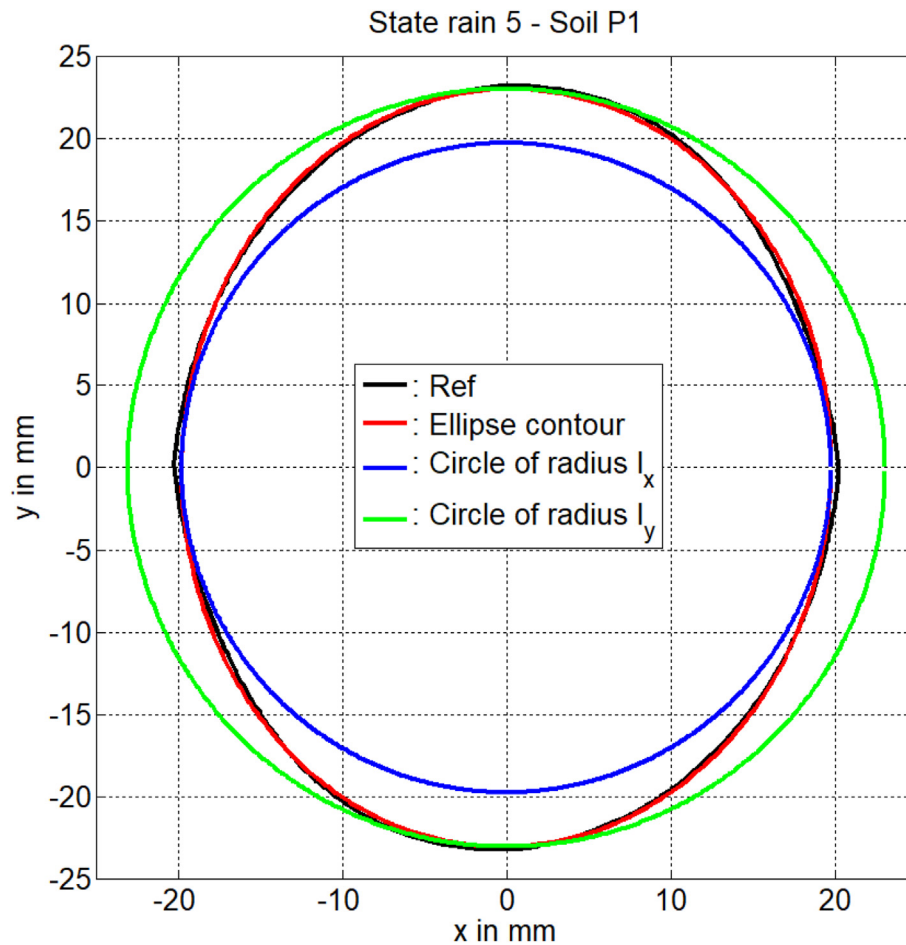
Fig. 3 – Level curve of reference autocorrelation function and ellipse or circles passing through correlation lengths for first laboratory soil surface at final state.
