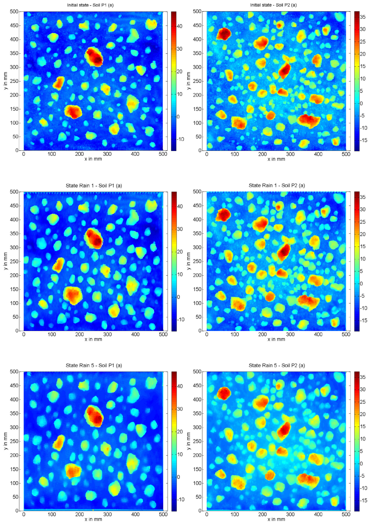
Fig. 1 – Top view of soil surfaces under study at initial state (top row), after first rainfall (middle row), after last rainfall (bottom row). Laboratory made soil surfaces with a low clod concentration (left column) and, with a high clod concentration (right column).
