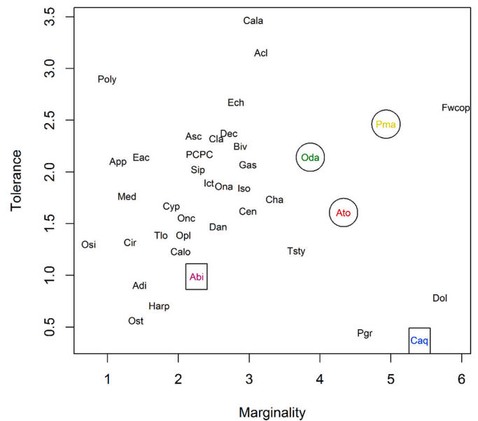
Fig. 4. Bivariate plot of all zooplankton taxa according to their marginality and tolerance. NIS and A. bifilosa and C. aquaedulcis copepods are shown inside circles and squares, respectively. Copepod taxa colours and abbreviations as in Fig. 2 and Table 1, respectively. (For interpretation of the references to colour in this figure legend, the reader is referred to the Web version of this article.)
