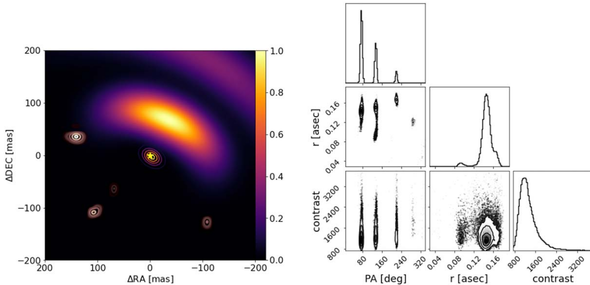
Figure 6. Left: the joint posterior density (copper contours) of the R.A. and decl. position of a companion when it was fit for, along with the two polar Gaussian ring plus inclined Gaussian model (background image + inclined Gaussian contours). Note that there are four potential locations for this planet found by the fitting. Right: corner plot showing only the companion components from the model fit. The four most likely localized spots are clearly identifiable in the PA vs. radius subplot.
