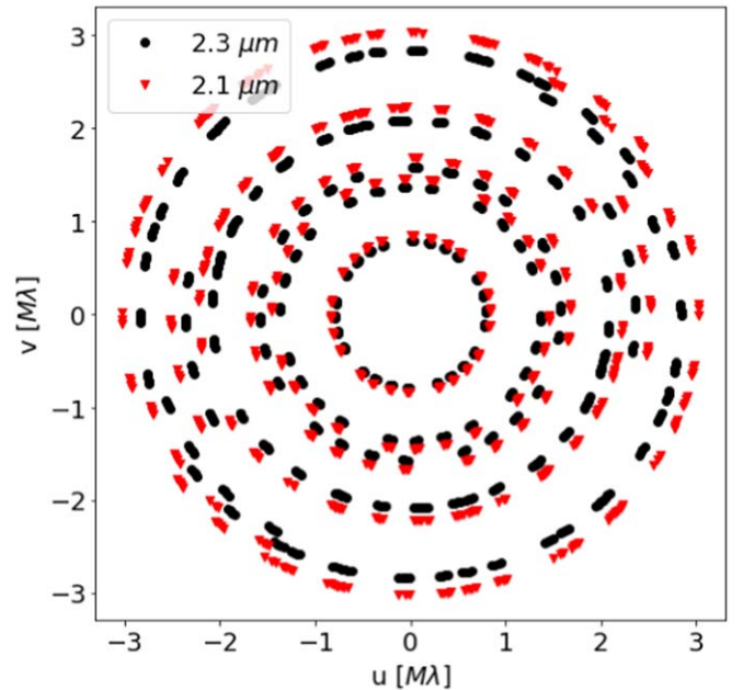
Figure 1. LkCa 15 VLT/SPHERE-IRDIS (u, v) -plane coverage. The largest and smallest baselines, B , correspond to spatial scales (\lambda/B) \sim 70 –260 mas (10–40 au).
