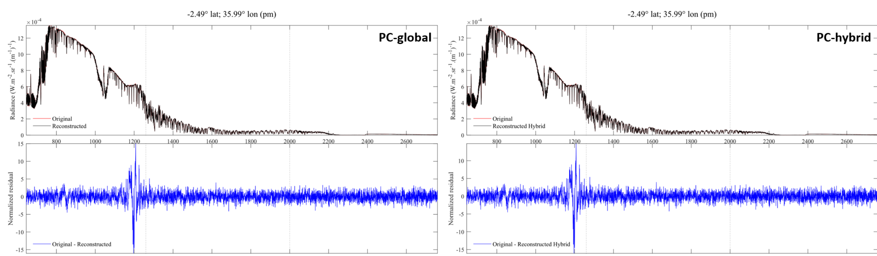
Original and reconstructed (with regular (left) and hybrid (right) approach) spectra of trona, thermonatrite and kogarkoite in absorption over the Lake Natron (2.49°S 35.99°E); and the difference.
