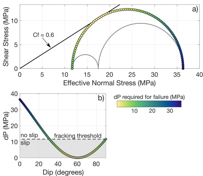
Figure 7. Minimum change in pore pressure ( dP ) required to reactive faults of specified dip. (a) Mohr circle and relative stresses for the Delaware Mountain group (Dvory & Zoback, 2021), assuming a coefficient of friction ( C_f ) of 0.6. (b) Minimum dP for slip as a function of dip. Any dP exceeding the fracking-threshold (dashed line in b) will produce new microfractures, significantly reducing the local effective stress. Thus, faults with orientations of dP greater than the fracking threshold are not expected to slip.
