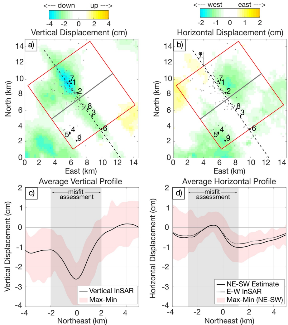
Figure 4. interferometric synthetic aperture radar (InSAR) results in selected study area. (a) Vertical and (b) east-west horizontal cumulative InSAR deformation, with relocated moment tensors (black, numbered dots) and earthquakes (gray dots). Within the red boxes, we calculated the average vertical and horizontal profiles along the gray line, perpendicular to the midline (dashed black line), which we assume to be the azimuth ( \phi ) of the predicted faults. The bottom panel shows (c), the average vertical profile, and (d), the average east-west horizontal and estimated northeast-southwest horizontal profiles. During modeling, we calculate the misfit within the shaded gray regions in (c) and (d).
