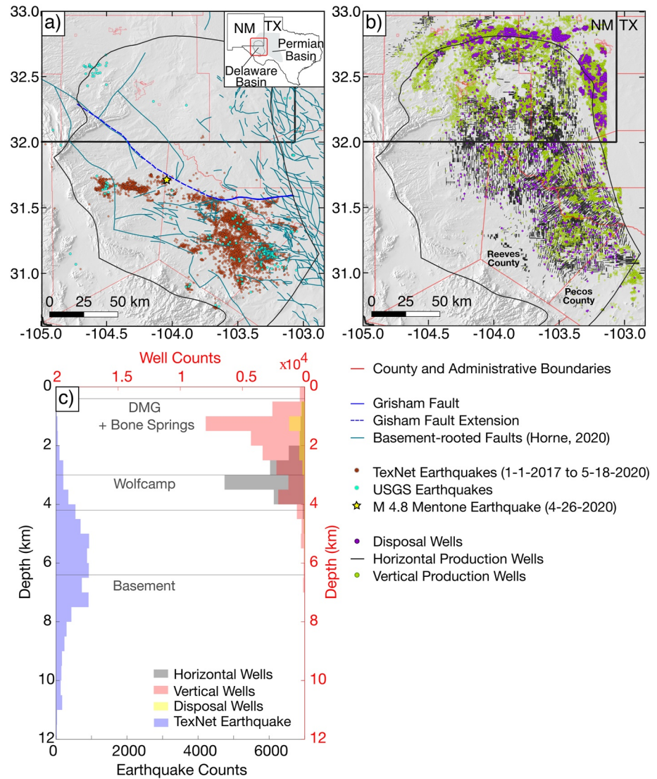
Figure 1. Seismicity, fault-mapping, and oil and gas activity in the Delaware Basin. (a) The seismic activity recorded by the USGS and TexNet arrays is concentrated in the southeastern Delaware Basin, below the Grisham Fault and its extension. Besides this distinction, few other faults show spatial correlations with seismic trends. (b) shows the disposal and productions wells that were active at some point between Dec 2014–June 2020 and assigned to the Delaware Basin (downloaded from Enverus, 1999). In contrast to the seismicity, oil and gas activity is widespread throughout the basin. (c) Earthquake depths from the TexNet catalog span a wide range, including into the basement, but these depths are highly uncertain. Most of the injection is concentrated above 3 km depth and above the producing shales. The formation depths depicted in (c) are approximate averages that we developed from formation surfaces provided by Enverus (1999); the true depth ranges vary throughout the basin. Fault traces provided by Horne, 2020.
