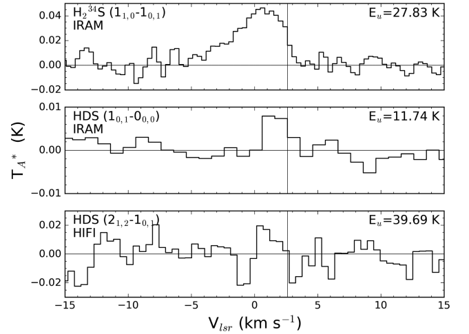
Figure 3. Herschel/HIFI and IRAM-30m/EMIR detections of H_2S isotopologues. The HDS lines are at lower spectral resolution than the other detections. The HDS ( 1-0 ) spectrum has a resolution of 1 \text{ km s}^{-1} and HDS ( 2-1 ) spectrum has a resolution of 0.5 \text{ km s}^{-1} .
