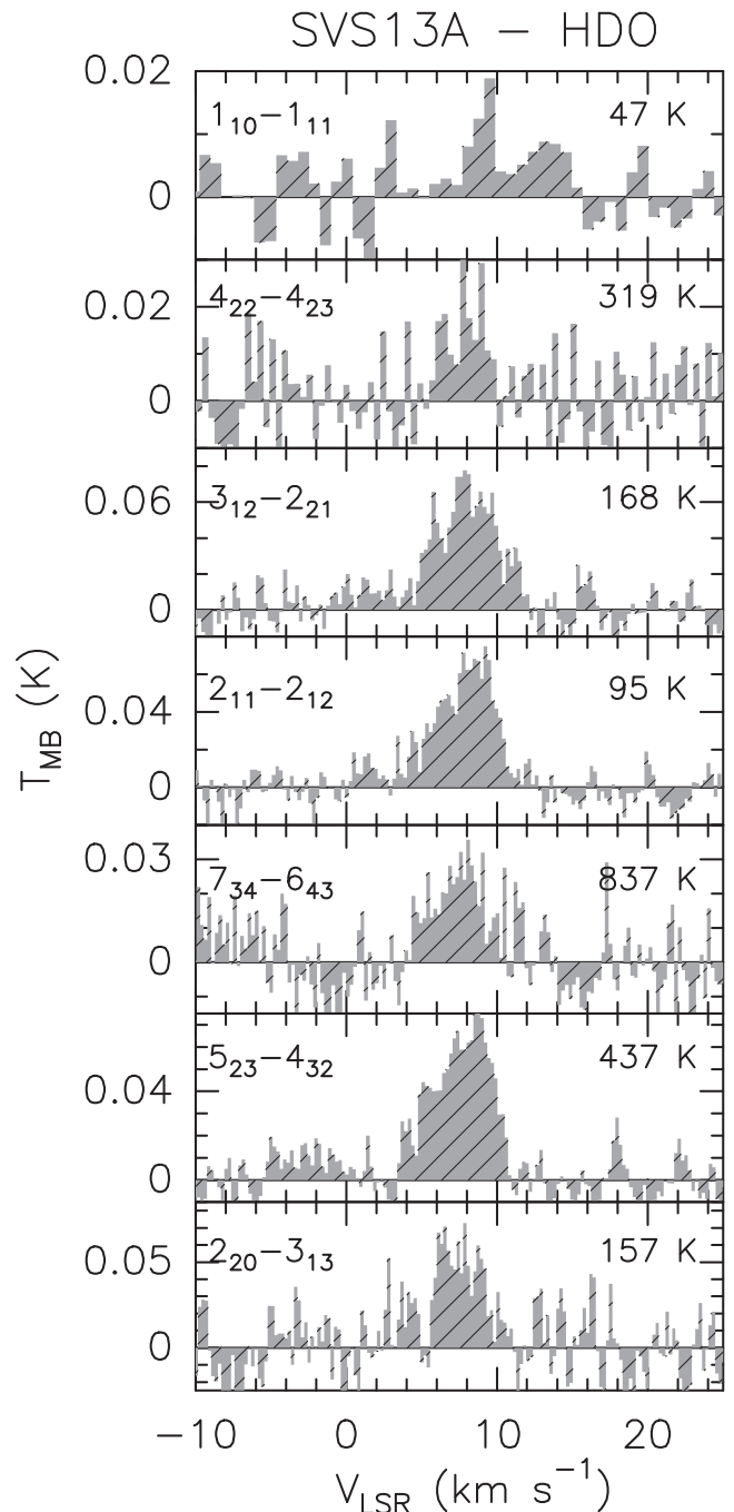
Figure 1. HDO line profiles (in main-beam temperature, T_{\text{MB}} , scale) observed with the IRAM 30-m antenna towards SVS13-A. In each panel, both the transition and the upper level energy, E_{\text{u}} , are reported.
