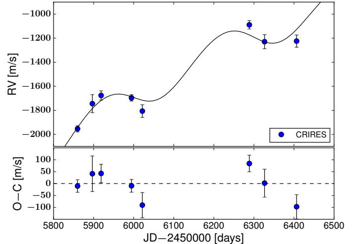
Fig. 3. Upper panel: CRILES infrared RV measurements of HD 59686 A. The black solid line shows the best Keplerian fit obtained from the Lick data alone. Bottom panel: residuals of the CRILES RVs from the optical fit. The value of the rms is \sim 59 \text{m s}^{-1} , which is consistent with the large infrared RV errors. The mean error of the CRILES data, with a jitter of 19.83 \text{m s}^{-1} added in quadrature, is \sim 45 \text{m s}^{-1} .
