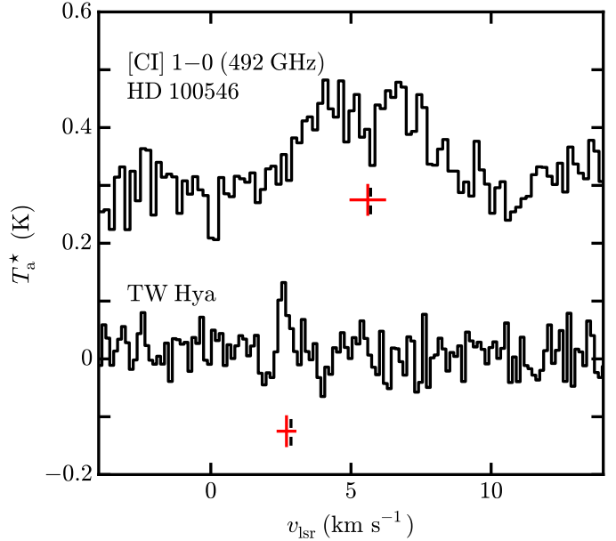
Fig. 1. [C I] 1–0 line in HD 100546 (offset by +0.3 K) and TW Hya. Horizontal bars mark the systemic velocities, 5.70 and 2.86 km s -1 . Red crosses show the best-fit Gaussian v_{\text{lsr}} with 3\sigma error bars. The data are binned to 0.14 km s -1 per channel.
