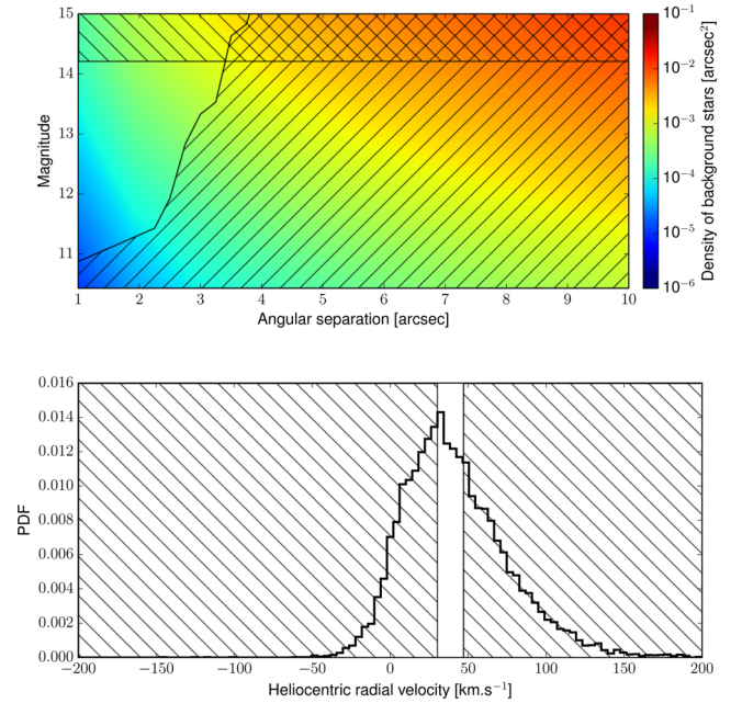
Figure 10. Upper panel: map of the density of background stars chance-aligned with WASP-121, integrated within an angular separation of up to 10 arcsec, as function of the V-band magnitude. The positive-slope hatched region displays all the stars that would have been significantly detected in the TRAPPIST data. The negative-slope hatched region displays the stars that are too faint to reproduce the observed transit depth of WASP-121. Lower panel: distribution of heliocentric RV of stars within 10^\circ from WASP-121 as observed by the RAVE experiment. The hatched regions show the velocity of background stars that should be spectroscopically resolved with WASP-121 and thus should produce a RV variation in antiphase with the transit ephemeris, or no significant variation (Santerne et al. 2015).
