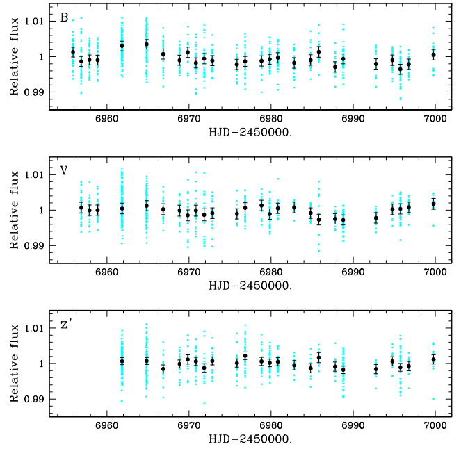
Figure 6. Out-of-eclipse photometric monitoring: globally normalized TRAPPIST differential photometry obtained for WASP-121 in Johnson-B (top), Johnson-V (middle), and Sloan-z' (bottom) filters, unbinned (cyan) and binned by day (black).
