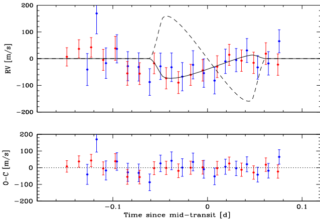
Figure 3. Top: zoom on the RM effect observed with CORALIE. The RVs obtained during the transit of 2014 Dec 24 are plotted in blue, while the RVs obtained during the transit of 2015 Jan 12 are plotted in red. The best-fitting circular Keplerian model (orbital motion) has been subtracted for clarity. The superimposed, solid black line is our best-fitting model for the RM effect. The dashed line is the RM effect that would have been observed in the case of an aligned orbit (shown for comparison). Bottom: residuals from our best-fitting model.
