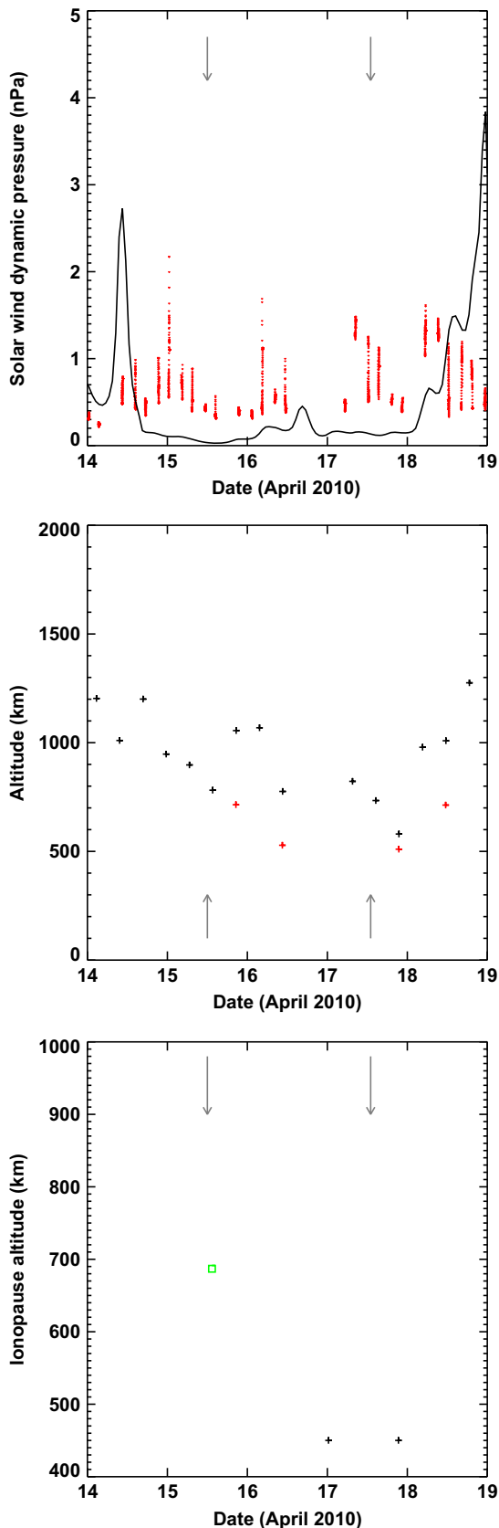
Fig. 10. As Fig. 8, but for case study C.
