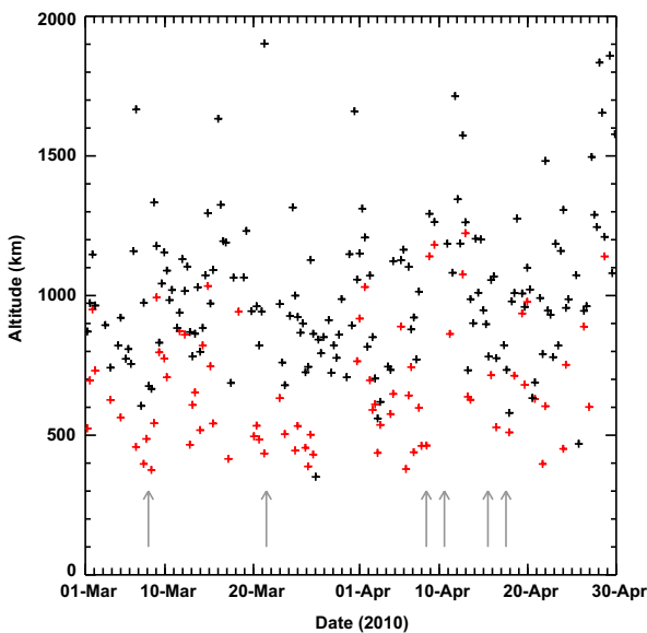
Fig. 4. Altitudes of the photoelectron boundary (red) and magnetic pileup boundary (black) on the outbound leg of the MEX orbit. Gray arrows mark the times of the six radio occultations (Section 4.1). (For interpretation of the references to color in this figure caption, the reader is referred to the web version of this paper.)
