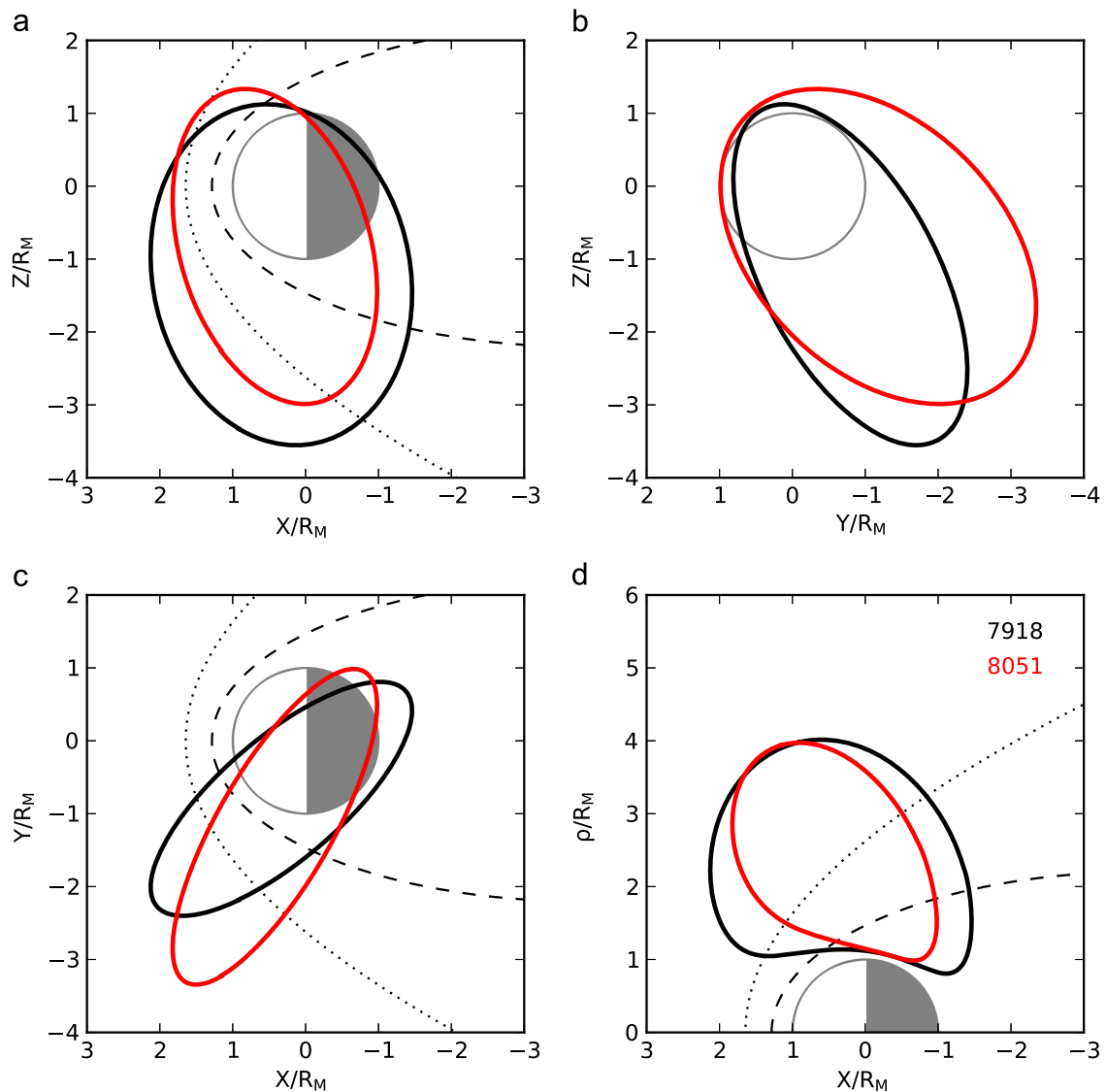
Fig. 2. MEX orbit geometry for 7 March (orbit 7918, black) and 15 April (orbit 8051, red) in Mars-centered Solar Orbital (MSO) coordinates. Modeled positions of the magnetic pile up boundary and the bow shock, according to Vignes et al. (2000) are also shown. Panel A shows the XZ plane, Panel B shows the YZ plane, and Panel C shows the XY plane. Panel D shows a cylindrical representation in which \rho^2 = Y^2 + Z^2 . (For interpretation of the references to color in this figure caption, the reader is referred to the web version of this paper.)
