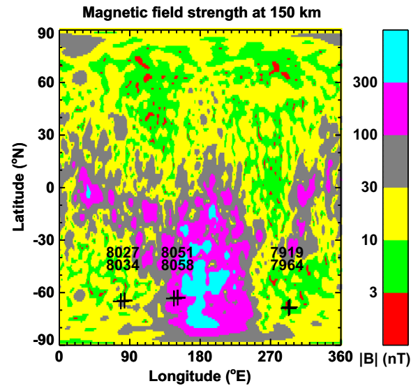
Fig. 5. Locations of six MEX radio occultation profiles (crosses). Pairs of numbers indicate the orbit numbers of each occultation. Also shown is the magnetic field strength at 150 km based upon the model of Arkani-Hamed (2004).
