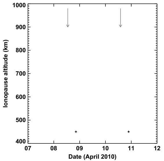
Fig. 9. As Fig. 8, but for case study B.
