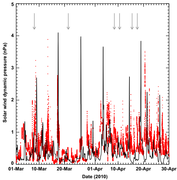
Fig. 3. Solar wind dynamic pressure measured at Mars by ASPERA (red) and extrapolated to Mars from STEREO-B (black). Gray arrows mark the times of the six radio occultations (Section 4.1). (For interpretation of the references to color in this figure caption, the reader is referred to the web version of this paper.)
