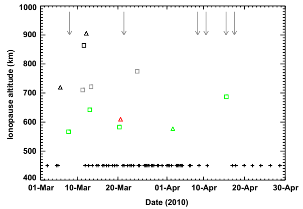
Fig. 7. Altitudes of abrupt changes in electron density detected in MARSIS local electron density data in March/April 2010. More abrupt changes, or those that would be classified as “ionopause” detections by Duru et al. (2009), are shown by squares and less abrupt changes are shown by triangles. Color indicates SZA: 65–70° as black, 70–75° as gray, 75–80° as red, and 80–85° as green. Orbits on which no abrupt change was detected are shown as black crosses at 450 km. Gray arrows mark the times of the six radio occultations (Section 4.1). (For interpretation of the references to color in this figure caption, the reader is referred to the web version of this paper.)
