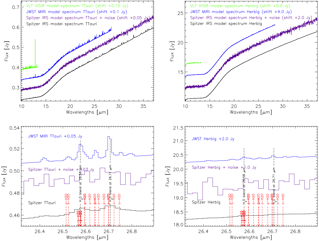
Fig. 9. Theoretical spectra convolved and re-binned at different resolutions ( Spitzer , IRS, R = 600 ; JWST MIRI, R = 3000 at 5.5 \mu\text{m} ; VLT VISIR, R = 25\,000 ), and zoom in the 26 \mu\text{m} region. The ranges adopted are the same as the instruments spectrographs. VISIR is ground-based, and the main limits are due to atmospheric transmission: we plotted only the region in which the transmissivity is \geq 80\% . The Spitzer spectrum with noise is also plotted in magenta. The strong feature at 12.93 \mu\text{m} in the VISIR modelled spectrum of a T Tauri star disk is due to \text{H}_2 ( J = 7-6 , v = 0 ). Water lines contributing to the blends at 26 \mu\text{m} are indicated by vertical red arrows.
