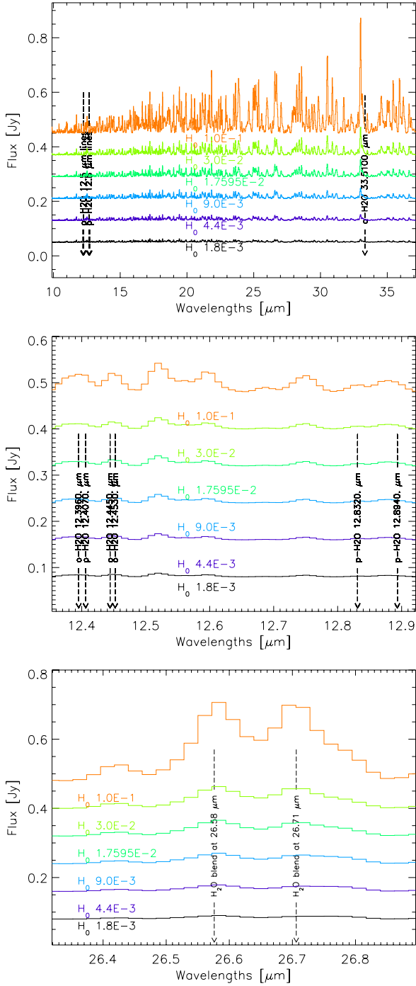
Fig. 6. Continuum-subtracted theoretical Spitzer spectra for H_0 variation, artificially shifted, convolved at the resolution of R = 600 , and rebinned. The second plot is a zoom of the complete spectrum on the 12 \mu\text{m} region. The third plot is a zoom on the 26.5 \mu\text{m} region.
