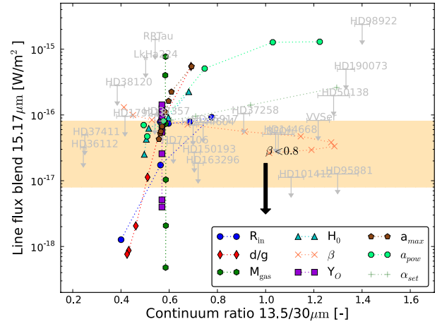
Fig. 7. Herbig parameter space for the water line blend at 15.17 \mu\text{m} . In the plot the data points (all upper limits, in grey) are from Pontoppidan et al. (2010a). All the fluxes are scaled to 140 pc. The shaded yellow area contains the range of sensitivity we retrieved from the Spitzer spectra of Herbig stars HD 135344B and HD 100546. All the fluxes of the disks considered are scaled to 140 pc. The trend toward disks being flatter than \beta = 0.8 is shown with a black arrow, since models that are too flat will be self-shadowed, and the derived mid-IR colour cannot be compared in a trustworthy manner with observations, in which the shadowing can be partial owing to a more complex disk structure.
