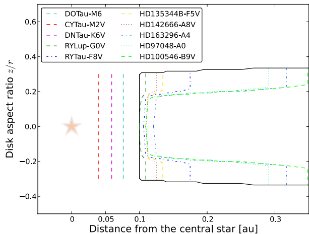
Fig. 4. Rockline position for the disks around different central stars. The thick black line indicates the disk contour at the gas density of 5 \times 10^3 \text{ cm}^{-3} for all our disk models, and we consider it as delimitation of our disk, because the erosion happens at more than 4 disk scale heights. The different colour and line styles delimit the contours of the disk with T_{\text{dust}} = 1500 \text{ K} assumed as sublimation temperature of silicates. Upward and inward of this contour, the dust is sublimated, and the disk is truncated. It describes the effective extension of the disk according to the dust sublimation temperature. For late type stars, disk temperatures are too low, and the contour is replaced by a vertical line that indicates the distance from which the dust in thermal equilibrium should be photoevaporated. The position of the central star is indicated by the star symbol.
