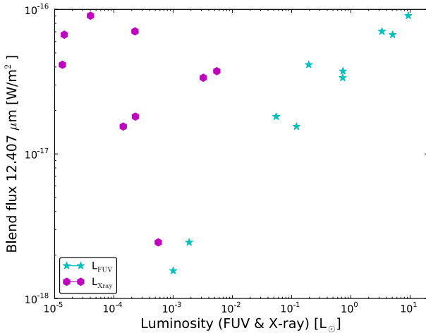
Fig. 2. Line fluxes for Spitzer 12.407 \mu\text{m} blend versus L_{\text{FUV}} (stars cyan) and L_{\text{X}} (magenta exagons).
