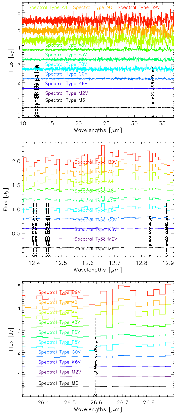
Fig. 8. Theoretical Spitzer SH/LH spectra ( R = 600 ) for models with different central stars rebinned and noisy; full continuum-subtracted spectrum, artificially shifted for all the models ( top ), zoom on the 12\ \mu\text{m} region ( middle ), zoom on the 26.5\ \mu\text{m} region ( bottom ).
