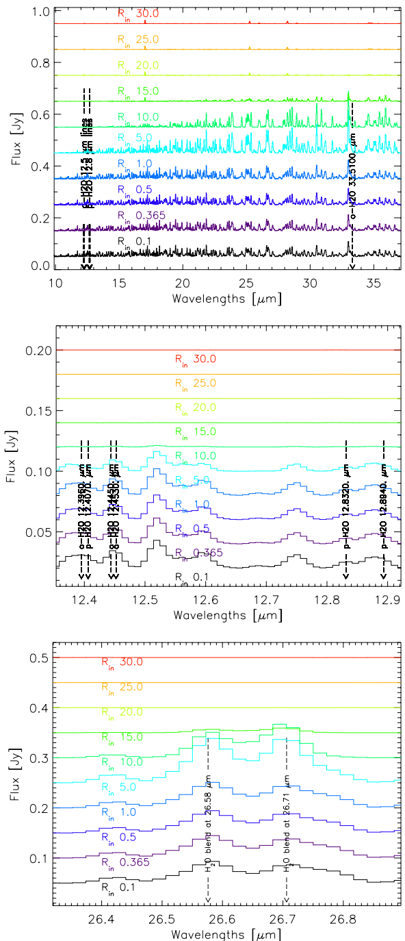
Fig. 5. Continuum-subtracted theoretical Spitzer spectra for R_{\text{in}} variation, artificially shifted, convolved at the resolution of R = 600 , and rebinned. The second plot is a zoom of the complete spectrum for the 12 \mu\text{m} region. The third plot is a zoom on the 26.5 \mu\text{m} region.
