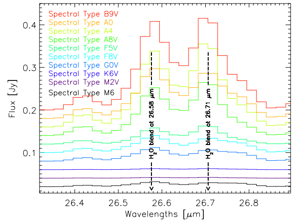
Fig. 3. Theoretical Spitzer SH/LH spectra (convolved at R = 600 and rebinned) for models with different central stars; full continuum subtracted spectrum, artificially shifted for all the models (top); zoom on the 12 \mu\text{m} region (middle); zoom on the 26.5 \mu\text{m} region (bottom).
