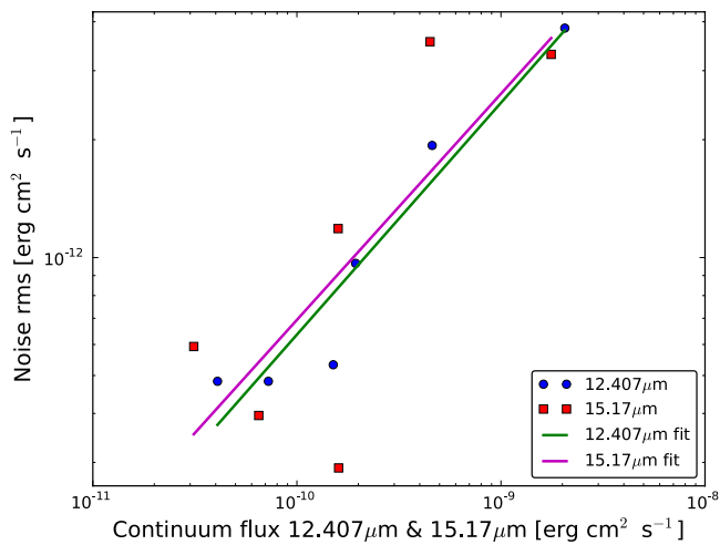
Fig. 11. Noise level versus continuum flux at the wavelengths of 12.407 \mu\text{m} (blue dots) and 15.17 \mu\text{m} (red squares). Overplotted are the fit to the data, green for 12.407 \mu\text{m} and magenta for the 15.17 \mu\text{m} .
