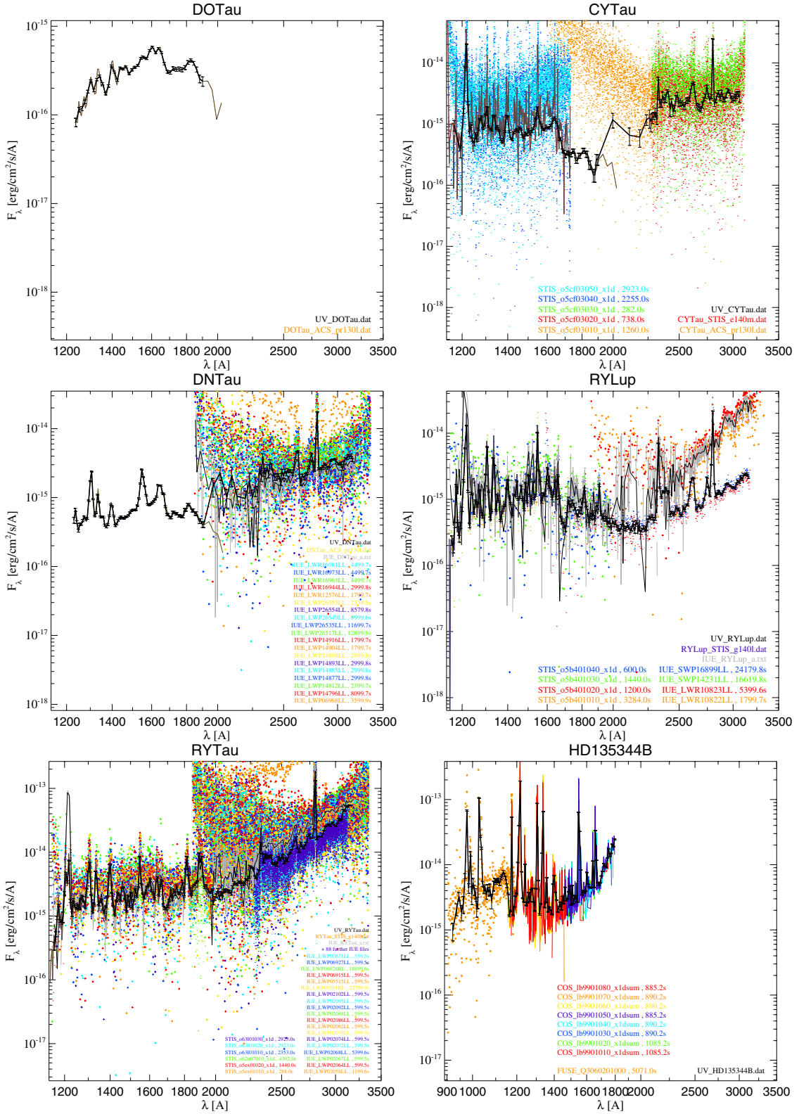
Fig. C.1. Far-UV component for each of the stars we modelled. The black line is the best fit of the multiple epochs of observations. Spectra data points are colour-coded, and the original files are labelled.
