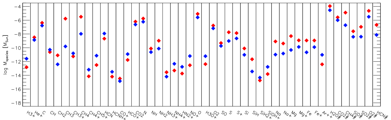
Fig. 16. Differences in species masses using the UMIST2012 database and its adsorption energies for the small (red, model 6) and large chemical network (blue, model 8).
