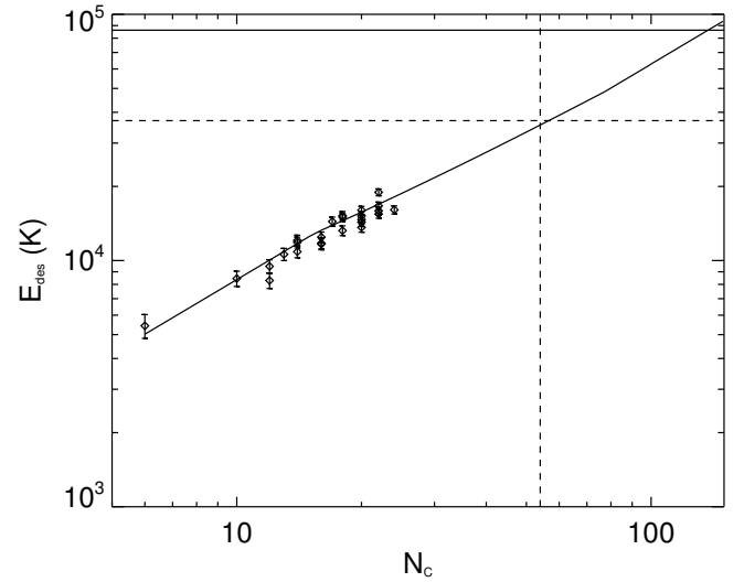
Fig. A.4. PAH desorption energy. The horizontal line corresponds to the limit imposed by the heat of vaporisation of graphite. The dashed-lines designate the desorption energy for circumcoronene ( N_c = 54 ).
