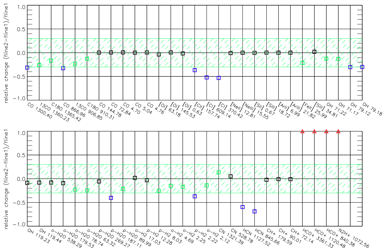
Fig. 17. Comparison of line fluxes using the UMIST2012 database and its adsorption energies for the small (flne1, model 6) and large chemical network (flne2, model 8). Black and green squares denote differences of less than 25% and less than a factor two respectively, blue squares and red triangles denote differences larger than a factor three and ten respectively.
