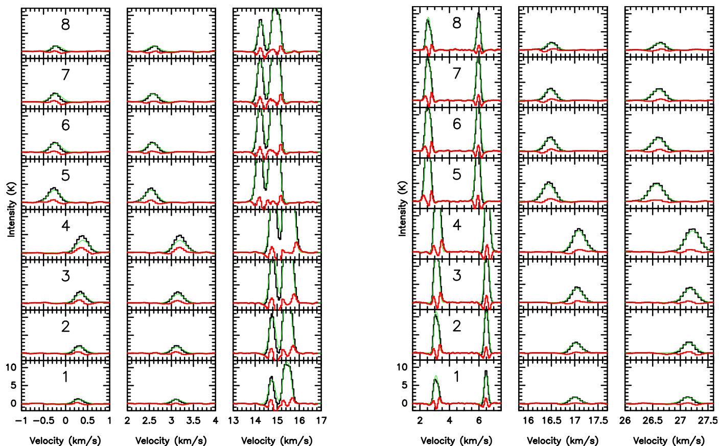
Fig. C.3. Spectra of the hf lines of CN ( a group, left ; b group right ) at different locations in the disk ( top panel ; integrated emission, in Jy/beam). Fits and their residuals to hyperfine structure (see Appendix C for details) are shown for each hf transition (green and red, resp.). Only reduced velocity intervals centered on the hf lines are shown.
