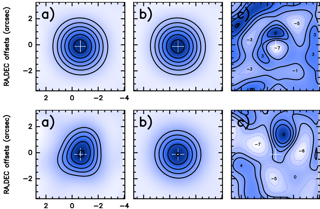
Fig. C.2. Results of the uv -plane analysis (see the text for details) for C^{14}N (top) and C^{15}N (bottom). On each row, panels a ) and b ) show the dirty image and the fitted Gaussian disk (Jy/beam), and panel c ) shows the residuals (in mJy/beam). For C^{14}N , contours in panels a ) and b ) are 0.1 to 0.7 by 0.1 Jy/beam, and for C^{15}N from 0.02 to 0.07 by 0.01 Jy/beam. Values of local extrema are indicated in the residuals. The C^{15}N fit assumes the Gaussian disk from C^{14}N . The results are summarized in Table 1.
