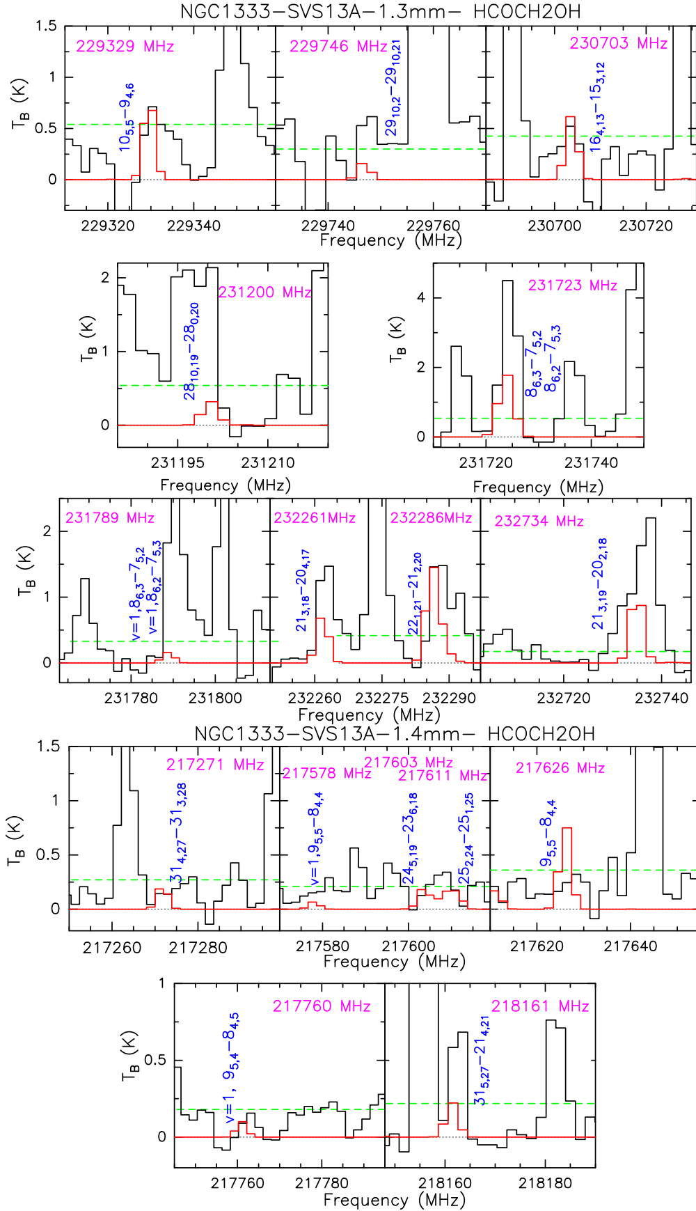
Fig. A.8. Glycolaldehyde emission lines (in T_B scale) observed in the 1.3 mm and 1.4 mm spectral windows towards NGC1333-SVS13A and excluded from the LTE analysis because of severe blending with other emission lines. The horizontal green dotted lines show the 3\sigma level. In blue we mark the glycolaldehyde transitions. The red line shows the synthetic spectrum obtained with the GILDAS-Weeds package (Maret et al. 2011) and assuming the rotation diagram solutions (see Fig. 3).
