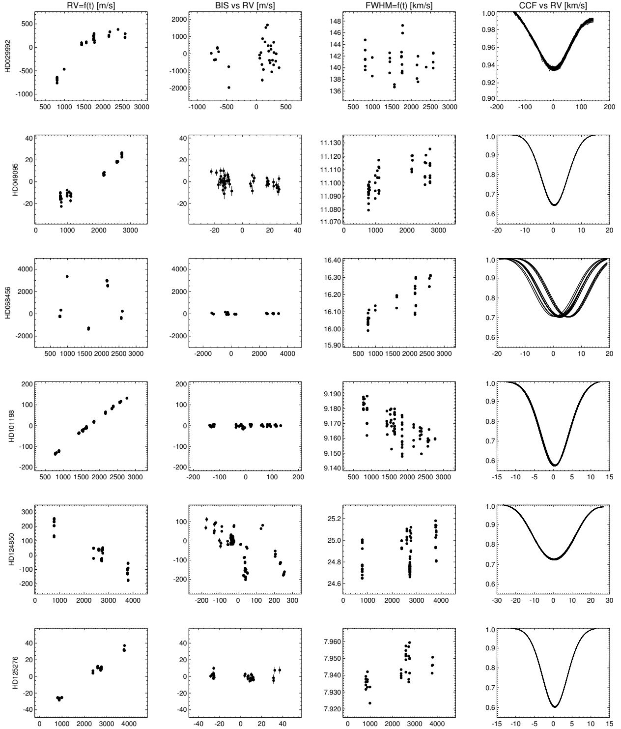
Fig. 6. Main HARPS data for our detected binaries (first part). From left to right: RV vs. time (Julian Day – 2 453 000), BIS vs. RV, FWHM vs. time, stacked CCF. From top to bottom: HD 29992, HD 49095, HD 68456, HD 101198, HD 124850, and HD 125276.
