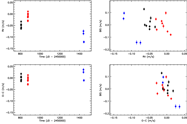
Fig. 5. Top: focus on HD 111998 RV data over 800 days ( left ) at three distinct epochs (black, red and blue dots); and corresponding (RV, BIS) diagram ( right ). Bottom: the same for HD 111998 RV residuals.
