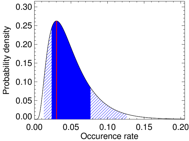
Fig. 14. Probability density function of the GP occurrence rate for planetary m_p \sin i in the range 1–13 M_{\text{Jup}} and for periods in the range of 1–1000 days, after correcting for the missed GP. Red: most probable value. Blue: 1\sigma confidence interval. Hatched blue: 2\sigma confidence interval.
