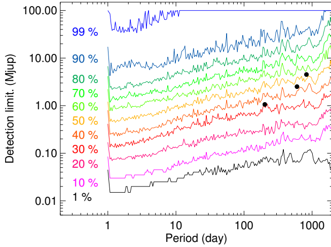
Fig. 13. GP search completeness of our survey. Black dots: detected GP ( m_p \sin i vs. P ). Solid lines: survey search completeness (i.e., fraction of stars with good enough detection limits to rule out planets of a given m_p \sin i at a given orbital period P ). From bottom to top: 1%, 10% to 90% (10% step) and 99% search completenesses.
