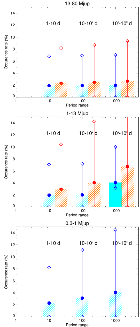
Fig. 15. Top panel: companion occurrence rate in the 13 to 80- M_{\text{Jup}} m_p \sin i range for three successive (non-cumulative) P ranges (from left to right: 1- to 10-day, 10- to 100-day and 100- to 1000-day ranges). Blue/cyan: M_\star \leq 1.5 M_\odot sub-sample. Red/orange: M_\star \geq 1.5 M_\odot sub-sample. Full color: occurrence rate computed in the case n_{\text{det}} \geq 1 . Shaded lines: occurrence rate computed in the case n_{\text{det}} = 0 . The 1\sigma confidence intervals are displayed for these two M_\star sub-samples as blue and red solid lines, respectively. Middle and bottom panels: occurrence rates for the 1- to 13- M_{\text{Jup}} and 0.3- to 1- M_{\text{Jup}} ranges, respectively.
