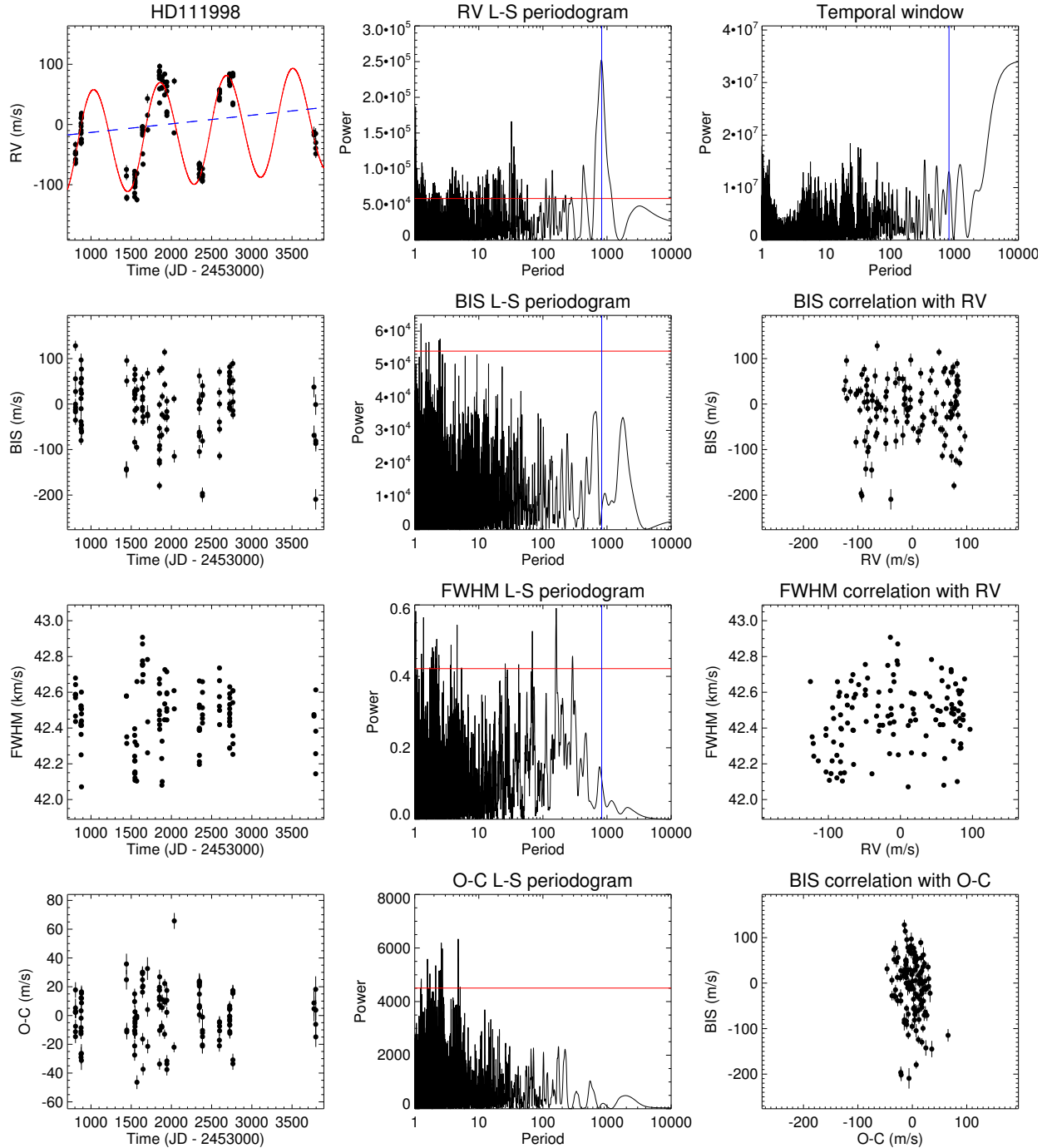
Fig. 4. Spectroscopic data for HD 111998. Top row: HD 111998 RV time series ( left ), RV Lomb-Scargle periodograms ( middle ) and temporal window of the observations ( right ). The Keplerian fit is superimposed (red solid line) to the RV, as well as the linear trend (dashed blue line). On the RV periodogram, the FAP at 1% (solid line) is indicated in red; the planet period is indicated in blue. Second and third rows: BIS and FWHM time series, corresponding Lomb-Scargle periodograms and correlations with the RV data. Fourth row: Residuals of the fit as a function of time, periodogram of the residuals and BIS correlation with the residuals.
