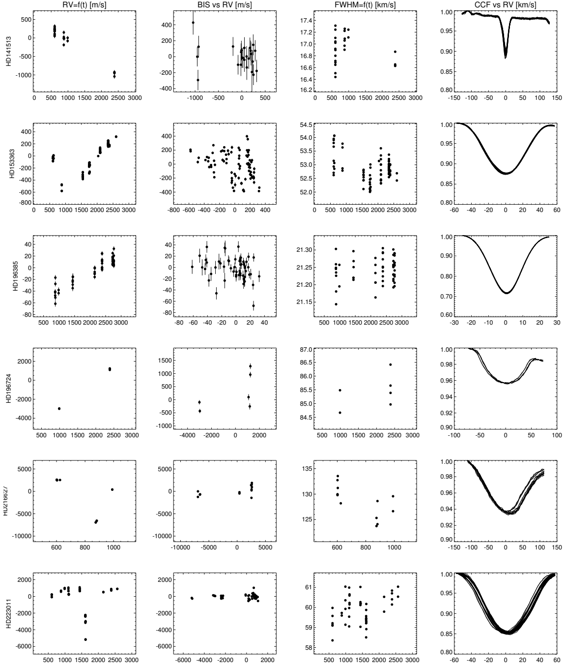
Fig. 7. Main HARPS data for our detected binaries (second part). From left to right: RV vs. time (Julian Day – 2453 000), BIS vs. RV, FWHM vs. time, stacked CCF. From top to bottom: HD 141513, HD 153363, HD 196385, HD 196724, HD 216627, and HD 223011.
