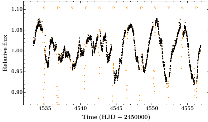
Fig. 3. CoRoT light curve from the 2008 observations. The out-of-eclipse data is shown in black and the stellar eclipses in orange (P and S indicate primary and secondary eclipses, respectively).
