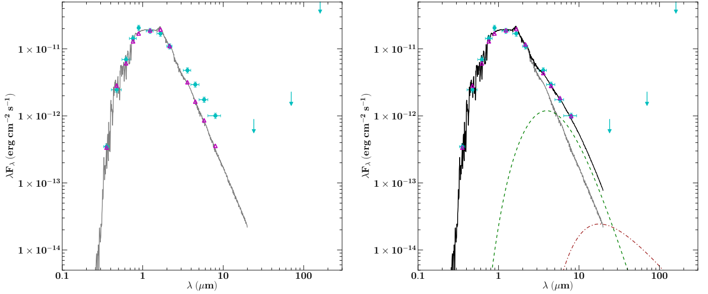
Fig. 1. Spectral energy distribution of CoRoT 223992193 (cyan points) with upper limits in the far-infrared (cyan arrows). This figure is identical to Fig. 13 of Gillen et al. (2014, Paper I); it is reproduced here for clarity. Left: the grey line and magenta triangles show the best-fit model using two naked stellar photospheres. Right: the black line and magenta triangles show the best-fit two naked photospheres model with a small amount of hot dust in the inner cavity of the circumbinary disk. The stellar and hot dust terms are shown separately as the grey solid and dashed green lines, respectively. Also shown for completeness, but not used in the fit, is the expected emission from a razor-thin circumbinary disk extending down to 22 R_{\odot} (brown dot-dashed line), which is illuminated by the central star and heated by the gravitational potential energy released from accretion with \dot{M} = 10^{-11} M_{\odot} \text{ yr}^{-1} .
