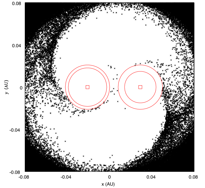
Fig. 14. Snapshot of the accretion flow structure in the corotating frame of the binary, as output from our particle model. The red squares indicate the locations of the primary and secondary stars (left and right, respectively) and the black crosses show the locations of particles in the circumbinary disk and the accretion streams onto the two stars. The red circles delimit the inner and outer edges of where dust could reside in circumstellar disks: the inner edge represents the sublimation radius for each star and the outer edge the radius at which the disks are truncated by the other star. The binary clears out a slightly eccentric cavity of radius \sim 0.08 – 0.1 AU ( \sim 17 – 22 R_\odot ).
