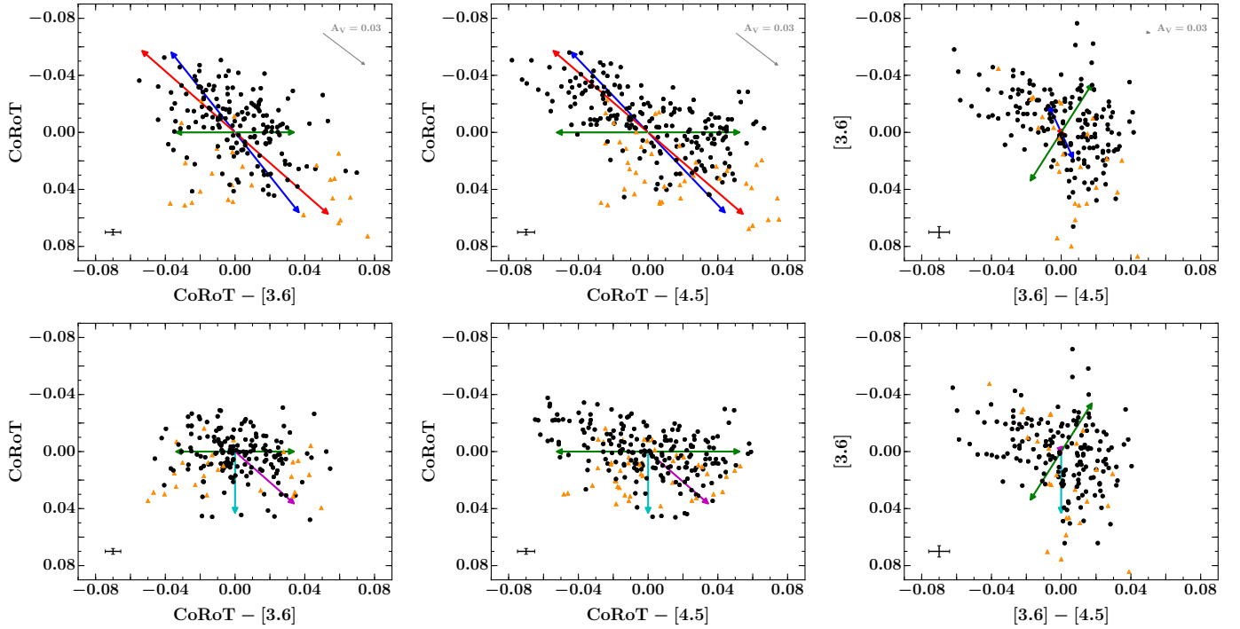
Fig. 9. Colour–magnitude diagrams. Top row, left to right: raw light curve data (black points) in the CoRoT vs. CoRoT-[3.6], CoRoT vs. CoRoT-[4.5] and [3.6] vs. [3.6]-[4.5] spaces. Data masked in the spot modelling are shown by the orange triangles. Coloured arrows show the effects of different types of variability: cold spots (blue), hot spots (red) and dust emission (green). Grey arrows indicate the direction of interstellar dust extinction. Bottom row, left to right: same as for the top row but showing the residuals of the spot modelling. Magenta and cyan arrows indicate the effects of obscuration by small and large dust grains, respectively. The error bar in the bottom left corner of each subplot shows a representative uncertainty for each data point. All plots share common axes.
