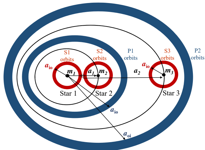
Fig. 1. Triple system with S-type and P-type orbits.
