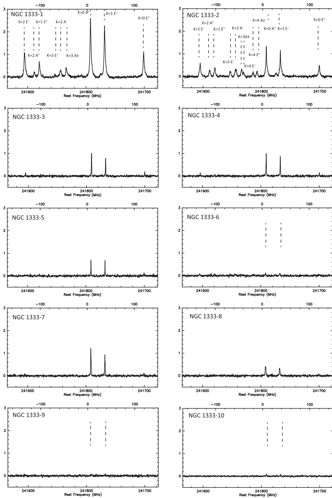
Figure 2. Line profiles of CH 3 OH ( J = 5-4 ) observed with IRAM 30 m. The spectra taken with the wobbler switching are indicated with an asterisk (ASAI project). (An extended version of this figure is available.)
