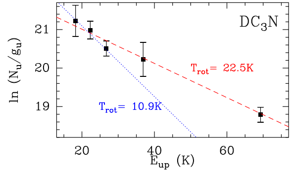
Figure A4. Rotational diagram analysis of DC 3 N emission. The emission was corrected for the coupling between the source and the telescope beam assuming a typical size of 20 arcsec. The best fit (dashed red line) is obtained for T_{\text{rot}} = 22.5 \pm 1.6 K and N(\text{DC}_3\text{N}) = (3.4 \pm 0.5) \times 10^{11} cm -2 . The fit obtained when considering only the data in the E_{\text{up}} < 40 K range yields T_{\text{rot}} = 10.9 \pm 1.7 K and N(\text{DC}_3\text{N}) = (5.2 \pm 1.8) \times 10^{11} cm -2 ; it is drawn by the blue dotted line.
