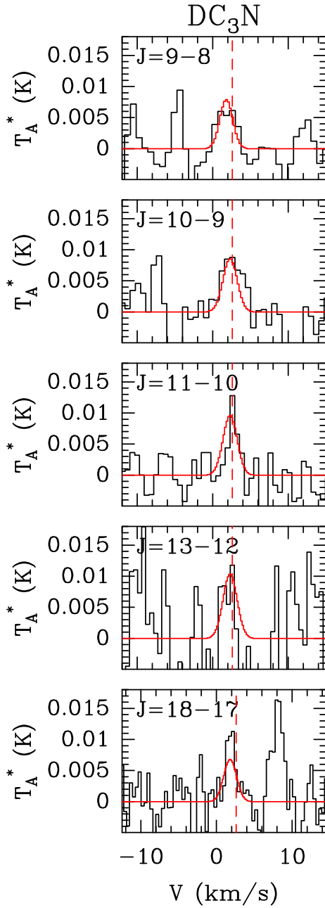
Figure A3. Montage of some DC 3 N lines detected towards L1157-mm. We have superposed in red the best LTE fit to the emission with T_{\text{rot}} = 22.5 \pm 1.6 K and N(\text{DC}_3\text{N}) = (3.4 \pm 0.5) \times 10^{11} cm -2 and a source size of 20 arcsec.
