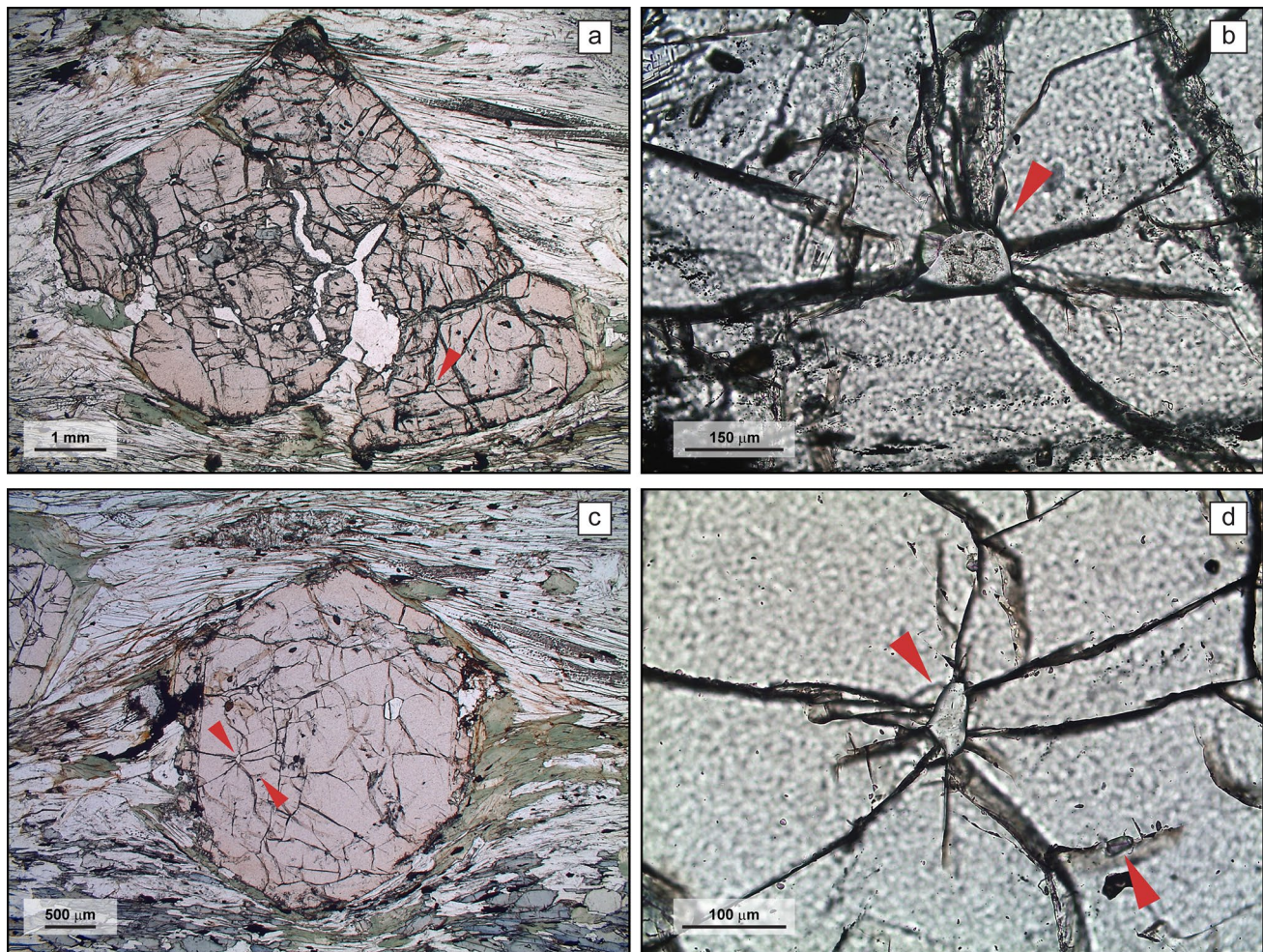
Fig. 4 Photomicrographs (plane-polarised light) for sample CH11. a Fractured garnet porphyroblast wrapped by the matrix foliation. Numerous inclusions of chloritoid, quartz, and rutile occur in the inner core, whereas garnet outer core displays only a few inclusions of coesite (red arrow) and rutile. Inclusions are almost absent in garnet rim, with the exception of a few rutile crystals. b Close-up of the coesite inclusion (partially transformed to quartz) enclosed in garnet, shown in (a). Note the radial fractures around the inclusion in the host garnet and the higher relief of coesite with respect to quartz. c Garnet porphyroblast with a coesite inclusion in the outer core (red
