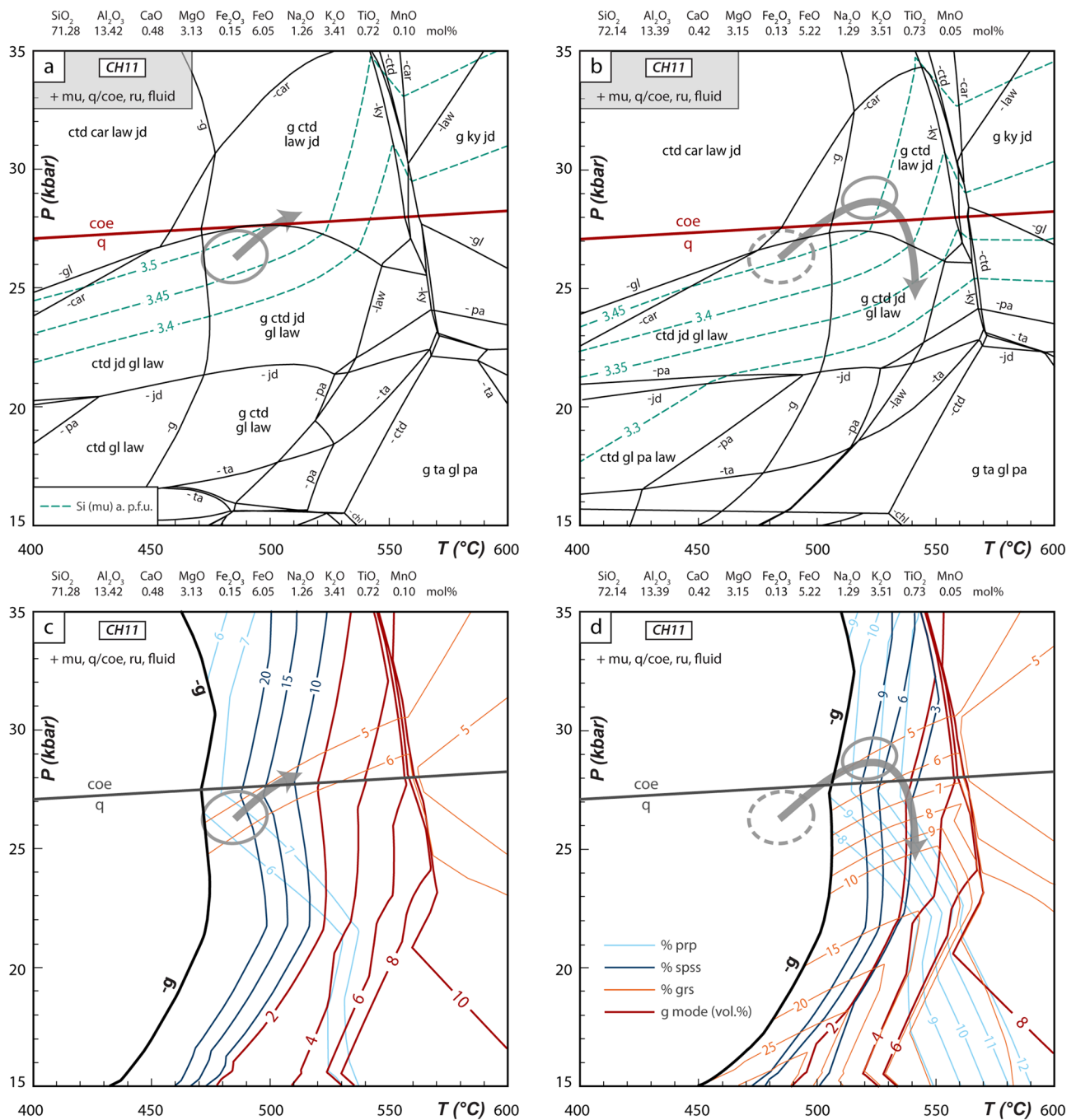
Fig. 10 \text{H}_2\text{O} -saturated P - T pseudosections calculated for sample CH11 using the unfractured bulk-rock composition (Tab. S6) (a) and a composition from which the garnet inner core has been subtracted (b). Some fields are not labelled for the sake of clarity; their assemblages can be deduced from the assemblages in adjacent fields.
