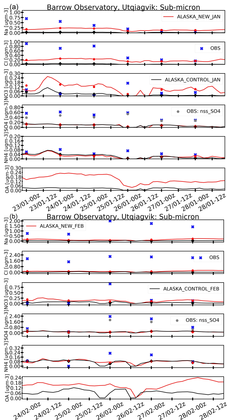
Figure 11. Time-series during a) January and b) February 2014 of sub-micron mass concentrations of Na + , Cl - , NO 3 - , NH 4 + , SO 4 2- , in \mu\text{g m}^{-3} , simulation period. Model simulations are validated against in-situ sub-micron aerosols at Utqiagvik, Alaska, in UTC (every 12h; 00z,12z). The black line shows model results from the CONTROL run; the red line shows the ALASKA_NEW run, while the daily observations are shown in blue crosses. The corresponding model daily averages are shown as black diamonds for the control simulation and as red pentagons for the ALASKA_NEW runs. See the text for details about the observations and model runs.
