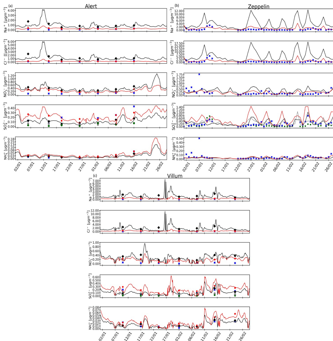
Figure 6. Evaluation of modelled aerosol composition against in situ aerosol observations with d_a < 10 \mu\text{m} in \mu\text{g m}^{-3} at (a) Alert, Canada (STP conditions); (b) Zeppelin, Svalbard; and (c) TSP aerosols at Villum, Greenland, in UTC. Observations are shown only when available. The lines and the symbols are the same as in Fig. 4. See the text for more details. Note the different scales.
