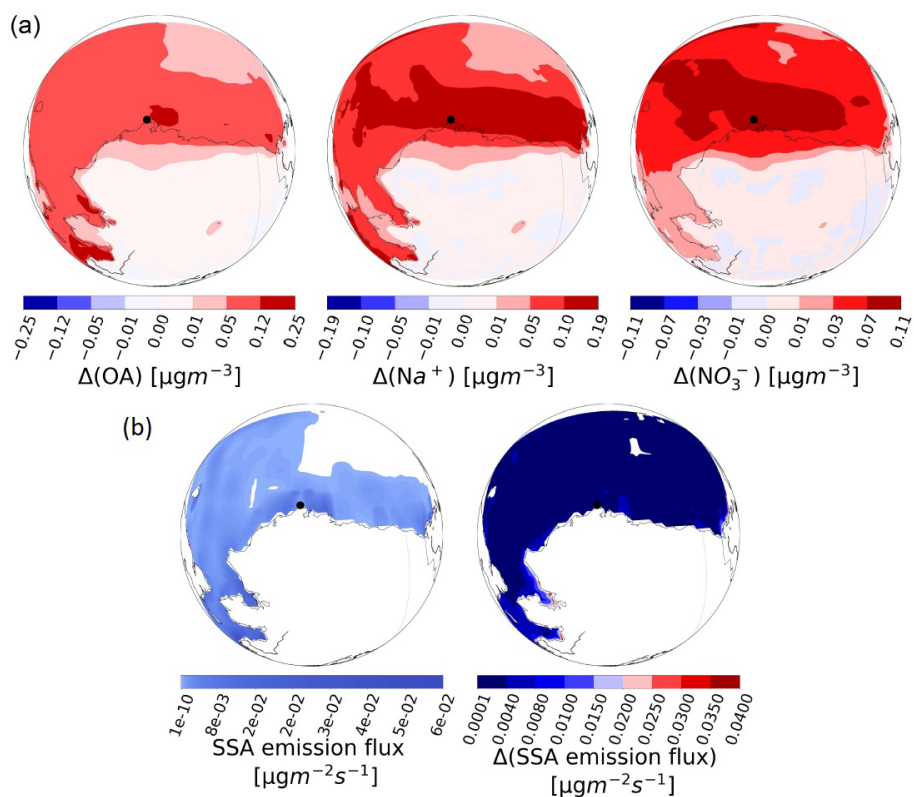
Figure 8. Average absolute differences in aerosol mass concentrations of (a) sub-micron \text{Na}^+ , OAs, and \text{NO}_3^- in \mu\text{g m}^{-3} between SSA_WS_DEP_FEB and LOC_ORG_FEB. (b) The map on the left shows the average value of SSA emission fluxes in \mu\text{g m}^{-2} \text{s}^{-1} during the February campaign, and the map on the right shows the average differences between SSA_WS_DEP_FEB and LOC_ORG_FEB emission fluxes in \mu\text{g m}^{-2} \text{s}^{-1} . All the results are shown at the surface. Utqiagvik is shown by the black dot. Note the different scales.
