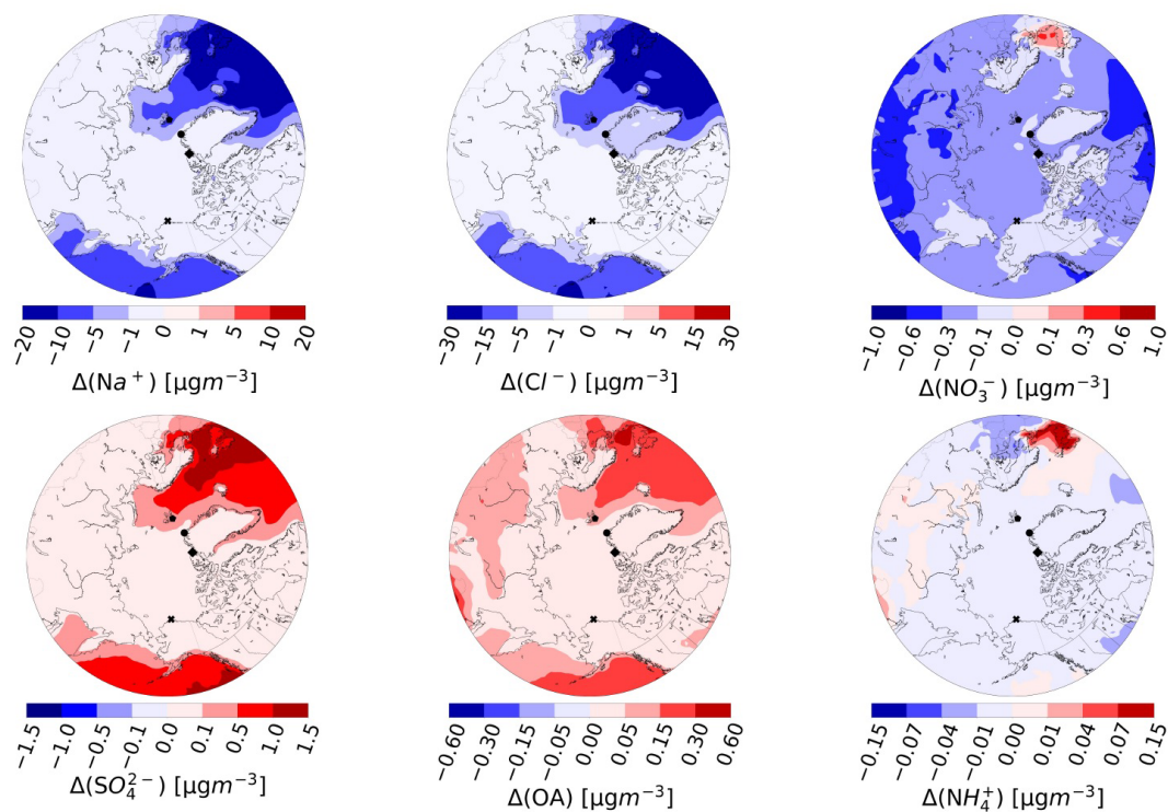
Figure 2. Average absolute differences in super-micron aerosol mass concentrations (in \mu\text{g m}^{-3} ) between HEM_NEW and CONTROL during January and February 2014 at the surface. The black \times in northern Alaska shows where Utqiagvik is located. The black circle shows Villum in Greenland; the black diamond shows Alert, Canada; and the black pentagon shows Zeppelin, Svalbard. Total \text{SO}_4^{2-} is shown. All the results are shown north of 50^\circ\text{N} . Note the different scales.
