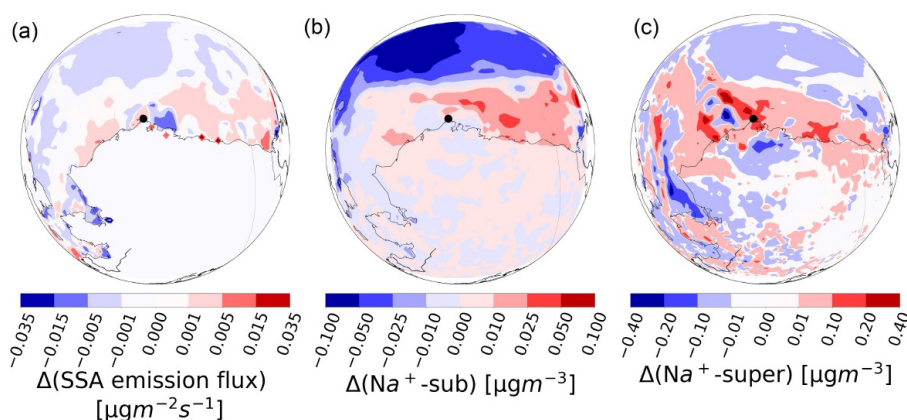
Figure 9. Average absolute differences between ALASKA_NEW_FEB and SSA_WS_DEP_FEB showing the effect of switching from FNL to ERA5 sea-ice fractions during the February campaign for (a) SSA emission flux ( \mu\text{g m}^{-2}\text{s}^{-1} ), (b) sub-micron \text{Na}^+ , and (c) super-micron \text{Na}^+ mass concentrations in \mu\text{g m}^{-3} . All the results are shown at the surface. Utqiagvik is shown by the black dot. Note the different scales.
