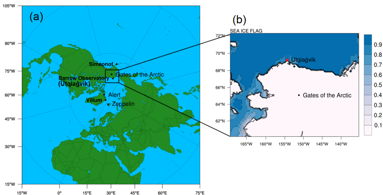
Figure 1. WRF-Chem simulation domains: (a) d01 is the 100 km domain, and (b) d02 is the 20 km domain. d02 shows sea-ice fractions interpolated at 20 km obtained from NCEP FNL at 1^\circ \times 1^\circ resolution (NCEP, 2000). See text for details.
