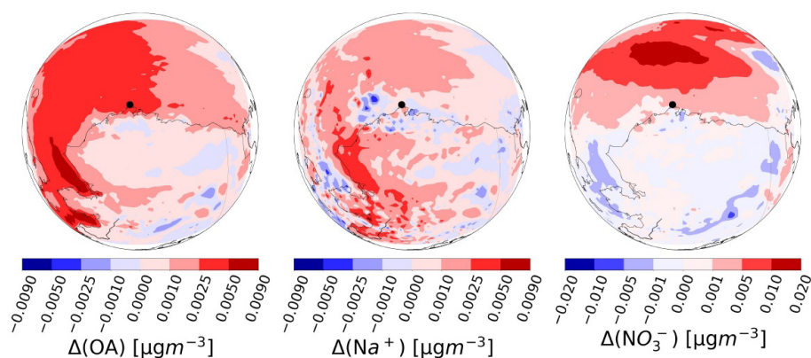
Figure 7. Average absolute differences in aerosol mass concentrations between LOC_ORG_FEB and ALASKA_CONTROL_FEB during the February campaign for sub-micron \text{Na}^+ , OAs, \text{NO}_3^- (in \mu\text{g m}^{-3} ). All the results are shown at the surface. See text and Table 4 for more details. Utqiagvik is shown by the black dot. Note the different scales.
