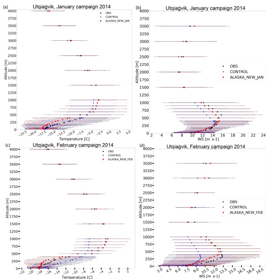
Figure E1. Average temperatures, in ^{\circ}\text{C} , and wind speeds (WS), in \text{m s}^{-1} , as a function of altitude (m) up to 4 km during the (a, b) January and (c, d) February campaigns in 2014 at Utqiagvik, Alaska. The radiosonde observations are shown as black circles. The blue pentagons show the model results for the CONTROL simulation (at 100 km), and the red diamonds show the model results for NEW_ALASKA_JAN and NEW_ALASKA_FEB. Observations are from IGRA2 and are available every 12 h (00:00 and 12:00 UTC). For the comparison, model output at 00:00 and 12:00 UTC is used. The corresponding horizontal lines show the standard deviations.
