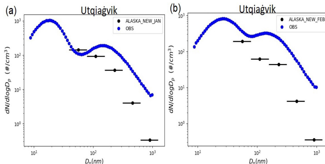
Figure 11. Averaged modelled (black) and measured (blue) particle number size distributions ( y axis) in particle number( \# )/ \text{cm}^{-3} during the (a) January and (b) February 2014 campaign periods at Utqiagvik as a function of particle diameter ( D_p ) in nm. The model results are from the ALASKA_NEW_JAN and ALASKA_NEW_FEB simulations. The black dot is plotted in the middle of each MOSAIC bin. The lines left and right of each dot indicate the minimum and the maximum of range of each bin.
