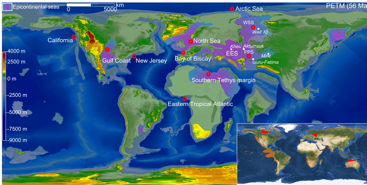
Fig. 1 Paleogeography during the PETM (modified from ref. 34). Until the Late Eocene isolation, the Eurasian Epicontinental Sea (EES) extended across Eurasia from the Mediterranean Tethys to the Tarim Basin in western China 17 . This study focuses on the central and eastern EES (delineated by black dashed line) consisting mostly of the West Siberian Sea (WSS) and the proto-Paratethys (PPS) that were connected via the Turgai Strait. Red circles show locations of the areas with enhanced organic carbon burial during the PETM (California and New Jersey 13 ; Gulf Coast 76,77 ; Bay of Biscay 80,81 ; North Sea 82,83 ; Eastern Tropical Atlantic 87 ; Southern Tethys margin 27 ; Arctic Sea 42 ; see also Table 2). Black dashed line indicates the study area with enhanced organic carbon burial in EES. The inset shows the modern day epicontinental seas (red triangles; Hudson Bay, Baltic Sea and Gulf of Carpentaria) and regions with high organic carbon concentrations (ca. 1.5% or more) in marine sediments (orange shaded regions, modified from ref. 51).
