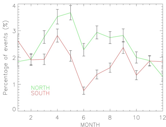
Figure 11. Percentage of events per month normalized by the number of registered half-orbits during the corresponding month for the Northern hemisphere (green) and the Southern hemisphere (red). The standard deviations are indicated by black bars.
