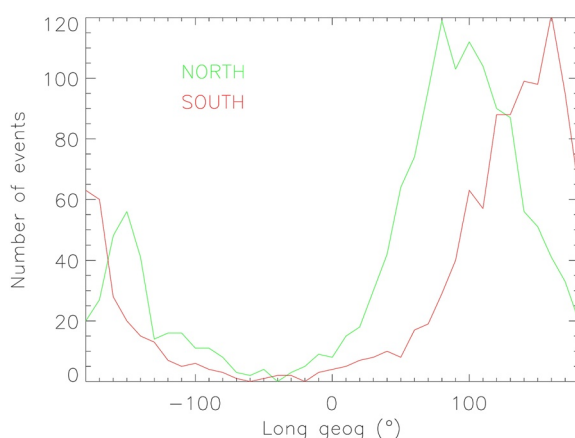
Figure 3. Number of events as a function of the geographic longitude in the Northern auroral zone (green) and in the Southern auroral zone (red).
