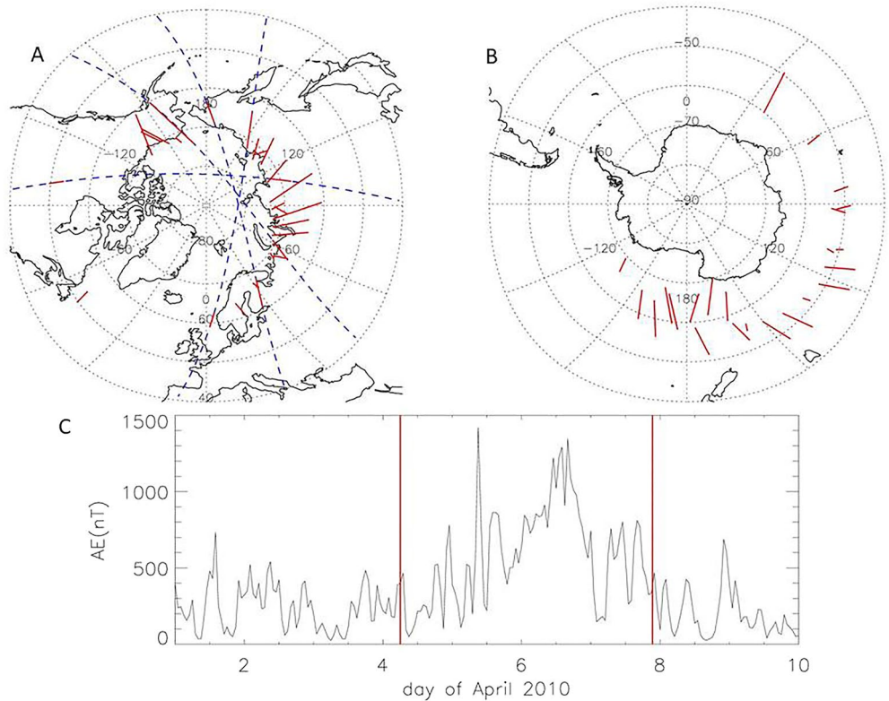
Figure 8. Sequence of 50 events (red segments) observed in the North (a) and in the South (b) between 4 April 2010 at 06:01 UT and 7 April 2010 at 21:23 UT at the time of a substorm indicated by the variation of the hourly AE index in panel (c) where the vertical red lines indicate the beginning and the end of this sequence of events. In the panel (a) the dashed blue lines indicate orbits where events are observed on each side of the auroral oval. The power spectrogram of one event is shown in the bottom panel of Figure 1.
