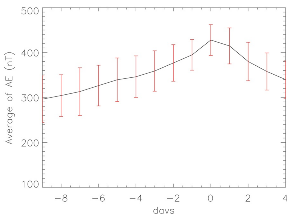
Figure 7. Average value of the AE index as a function of the days before and after the 2,526 events. The standard deviations are indicated by red bars.
