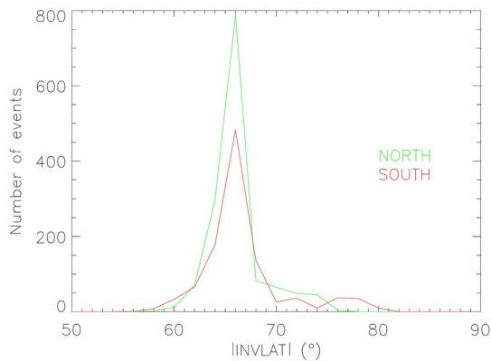
Figure 10. Variation of the number of events as a function of the invariant latitude in the North hemisphere (green) and in the South hemisphere (red).
