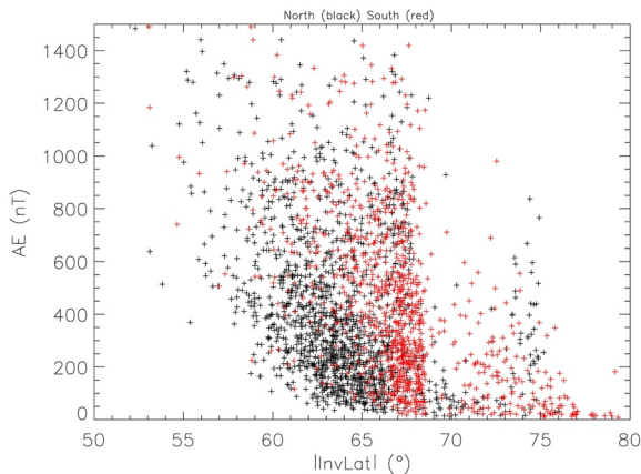
Figure 6. Variation of the invariant latitude of the events as a function of the AE index in the Northern hemisphere (black sign +) and in the Southern hemisphere (red sign +).
