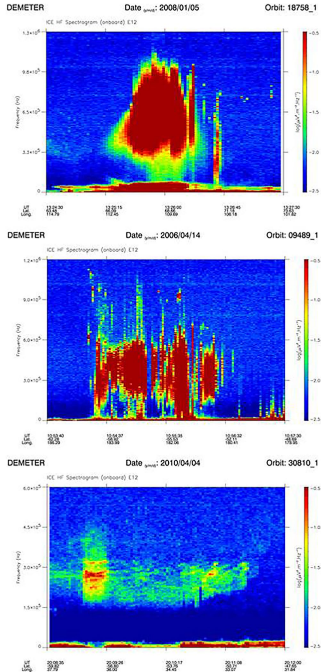
Figure 1. Examples of auroral kilometric radiation-like emissions observed by DEMETER. (top panel) emissions recorded on 5 January 2008 between 13:24:30 and 13:27:30 UT in the frequency range 0–1.3 MHz; (middle panel) emissions recorded on 14 April 2006 between 10:53:40 and 10:57:30 UT in the frequency range 0–1.2 MHz; (bottom panel) emissions recorded on 4 April 2010 between 20:08:35 and 20:12:00 UT in the frequency range 0–600 kHz. The intensity of the emissions is color coded according to the scale on the right of each panel. The parameters at the bottom of each panel are the geographic latitude and longitude.
