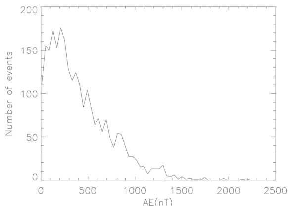
Figure 5. Number of events as a function of the substorm AE index.
