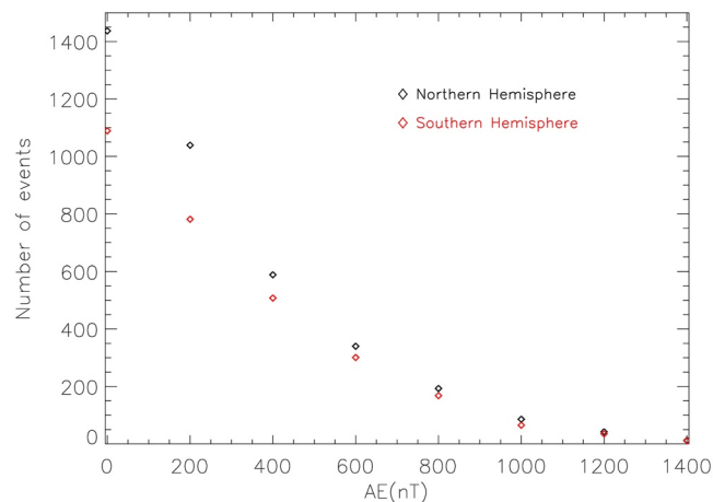
Figure 14. Number of events in the North (black diamond) and in the South (red diamond) when AE is larger than the value indicated on the horizontal axis.
