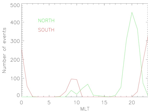
Figure 9. Number of events as a function of magnetic local time in the Northern hemisphere (green) and in the Southern hemisphere (red).
