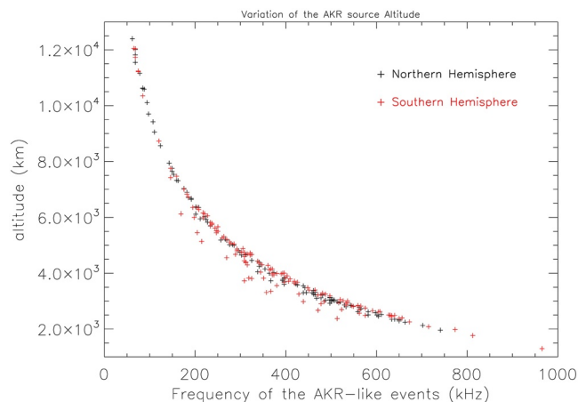
Figure 13. Variation of the source altitude of the expected parent auroral kilometric radiation (AKR) as a function of the frequency of the AKR-like events for the North (black +) and the South (red +). See text for explanation.
