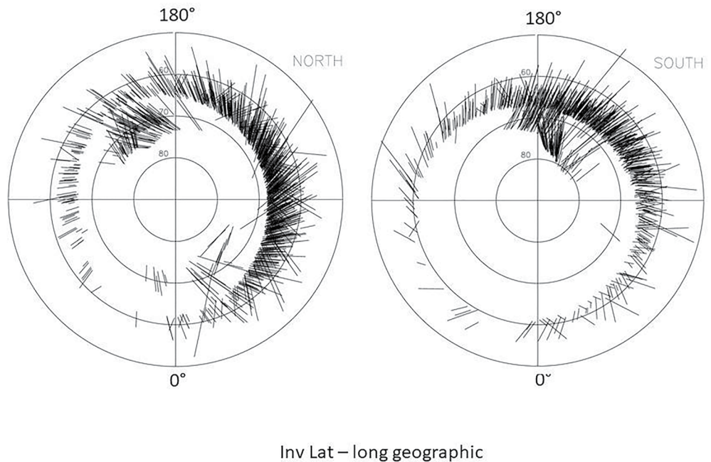
Figure 4. Same data as in Figure 2 but displayed in two polar plots as a function of the invariant latitude and the geographic longitude in the Northern (left) and Southern (right) hemisphere.
