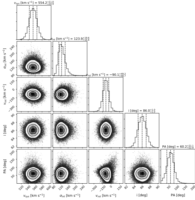
Fig. 1. Posterior distribution of the five fitting parameters from the MCMC analysis of the Cen A satellite system. In the histograms, the three dashed lines indicate the 16, 50, and 84 percentiles, which correspond to the upper and lower uncertainty boundaries, and the best-fit parameter estimation (i.e., the median). See Sect. 2 for details.
