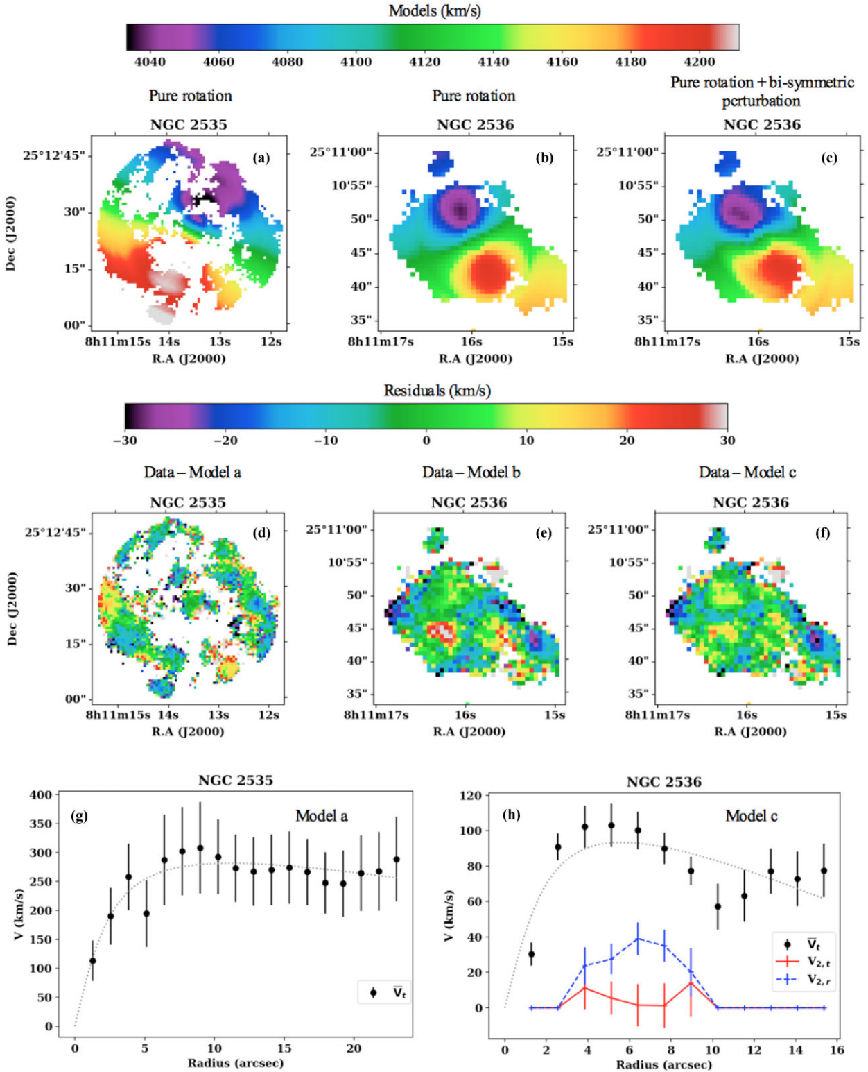
Figure 5. Fitted velocity models for the H\alpha velocity fields. (a)–(c): Rotation-only models for NGC 2535 and NGC 2536 and rotation + bisymmetric flow model for NGC 2536. (d)–(f): Corresponding residuals. (g) and (h): Rotation curves correspond to the best-fitting models, i.e. rotation-only model for NGC 2535 and rotation + bisymmetric flow for NGC 2536. The dotted lines are arctan functional fits to the rotation curves (see text).
