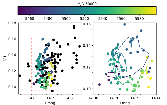
Fig. 21. J0524: OGLE V – I colour index vs. I (interpolated linearly to the times of the V -band measurements). Left panel : we plot the complete data set. Right panel : we restrict the times to MJD 55400–55600 (see shaded region in Fig. 20). Apart from a general trend of redder when brighter, smoothing the date reveals a hysteresis loop (see right panel ), where the rise of a flare is bluer than the decay.
