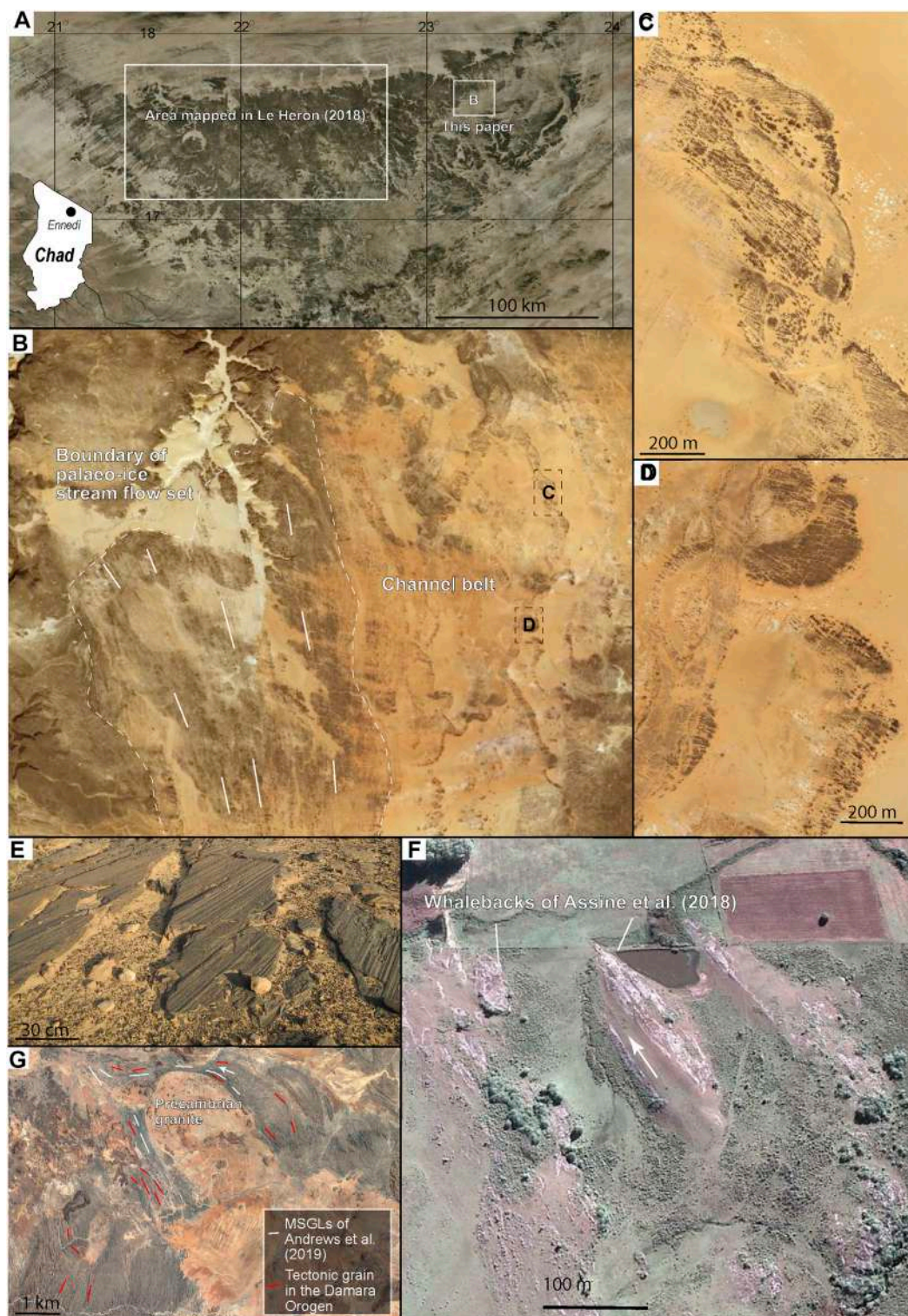
FIGURE 3 | The interpretation of Late Palaeozoic Ice Age (LPIA) glacial land surfaces from satellite data. (A) The Ennedi plateaux of northern Chad, showing the mapped location of the palaeo-ice stream network documented in Le Heron (2018), and its eastward continuation (this study). (B) Interpreted palaeo-ice stream flow set with mega-scale glacial lineations (MSGLs) to the left of the image, and an extensive channel belt to the right. The location of the images (C,D) are highlighted in the small rectangles. (E) Soft-sediment striations at outcrop in the Ennedi plateaux. Image courtesy of Ursula Steiner, whose photo was taken at 17.623°N 22.777°E. (F) Google Earth image of whalebacks published in Assine et al. (2018) - hard bedrock structures in the LPIA of northern Uruguay. See Assine et al. (2018) for precise location information. (G) The zone of the Damara Orogen, central Namibia, featured in Andrews et al. (2019). These authors interpreted MSGLs, yet here we caution that these are parallel to the tectonic grain of the orogen, underscoring that the utmost care must be taking when mapping and interpreting deep time glacial land surfaces from satellite imagery. See Andrews et al. (2019) for precise location information.
