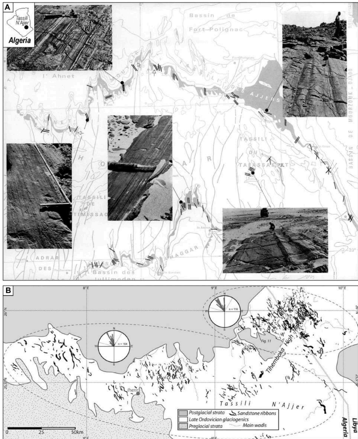
FIGURE 1 | Historical successes in capturing big picture glacial geomorphology in the ancient record. (A) The mapping efforts of Beuf et al. (1971) are a landmark achievement in the documentation of the Late Ordovician glacial record of southern Algeria. This map (reproduced with permission) shows the distribution of soft-sediment striated surfaces across the Tassili N'Ajjer (shown here as the Tassili des Ajjers) plateau (represented by simple, black parallel lines). These authors did substantial fieldwork in the region, and the photos show five separate examples of these soft-sediment striated surfaces over a wide area. (B) Mapping in the Tassili N'Ajjer 40 years later (Girard et al., 2012), with focus of meltwater structures (sandstone ribbons in this image). The impressive, dense network of structures results from high fidelity aerial photograph and satellite image mapping made possible thanks to the undeformed nature of the substrate, the gently dipping plateau, and the lack of vegetation in the central Sahara. Reproduced with permission of the Geological Society of London.
