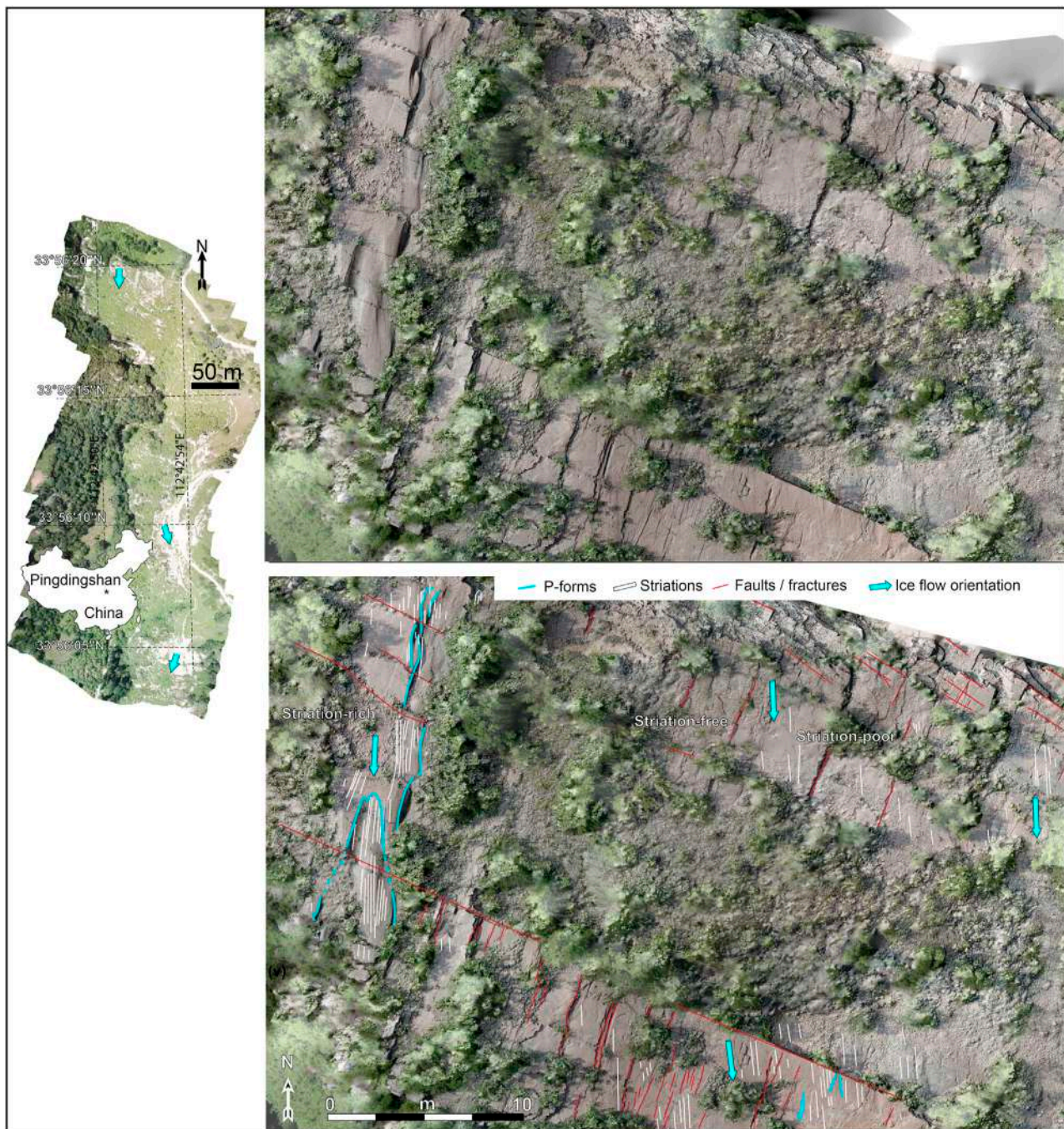
FIGURE 4 | The Pingdingshan striated pavement of Ediacaran age, central China, from Le Heron et al. (2019a). The image derives from data collected by a DJI Mavic Pro UAV in June 2018 as follows. A semi-transparent orthophoto has been draped over a digital elevation model to that small scale topographic differences are emphasised, thereby assisting geomorphic mapping. The abundance of p-forms on this surface highlights the role of subglacial meltwater is sculpting m-scale topography into lithified sandstone basement.
