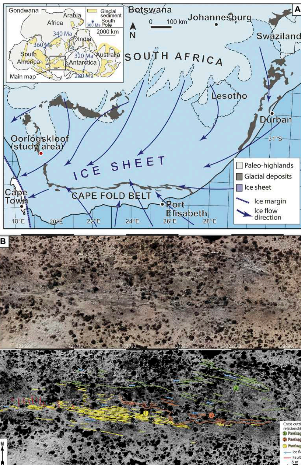
FIGURE 5 | (A) Paleogeographic map of South Africa during the late Paleozoic ice age, and outline of ice-sheet flow character, based on Visser (1997), Lopez-Gamundi and Buatois (2010). Study area at Oorlogskloof is situated at the western margin of the Karoo Basin. (B) Bird's eye view of the Oorlogskloof glacial pavement of South Africa (top) together with an interpretation of the surface and the recognition of cross-cutting relationships (bottom). The bird's eye view consists of drone data, namely an orthophoto layered over a digital elevation model. From Le Heron et al. (2019b).
