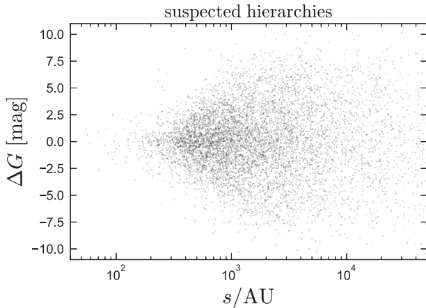
Figure 17. Magnitude difference between the two resolved components of all wide binaries in which one or both components is suspected to have a bright, unresolved companion ( N = 7, 295 ; yellow points in Fig. 1). There is no obvious excess at \Delta G \approx 0 (compare to the right-hand panel of Fig. 3).
