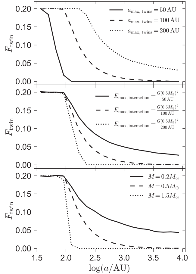
Figure 16. Predictions of the toy model for orbit widening described in Section 5.2.1. We assume that the initial twin fraction is 20 percent for a < a_{\text{twin, max}} (varied in the top panel; 100 au by default) and 0 at larger separations. We consider an initial separation distribution that is flat in log space. We then widen the orbits of all binaries by adding energy, representing the cumulative effect of gravitational interactions within a birth cluster. The total added energy is drawn from a uniform distribution between 0 and E_{\text{max, interaction}} . Binaries that are disrupted are discarded. We plot the final twin fraction as a function of separation, varying E_{\text{max, interaction}} (middle panel; default is G(0.5M_{\odot})^2/(100 \text{ au}) ) and mass (bottom panel; default is 0.5 M_{\odot} ).
