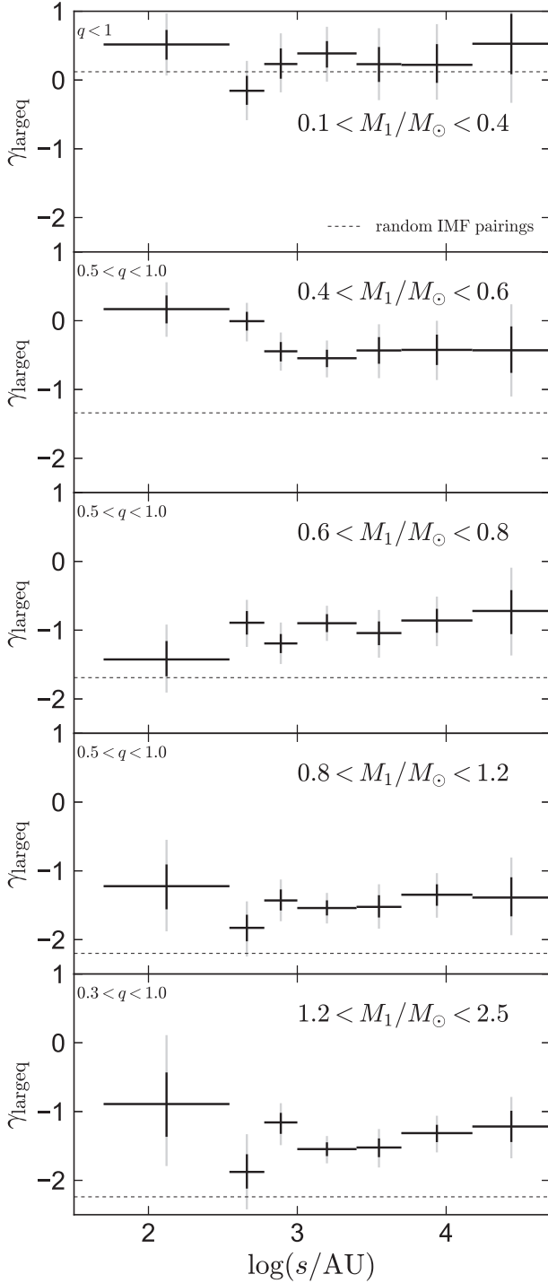
Figure 12. Marginalized constraints on \gamma_{largeq} , the logarithmic slope of the power-law component of the mass ratio distribution at large q , versus projected separation. Dark and light error bars show 1\sigma and 2\sigma constraints. The range of q over which \gamma_{largeq} is fit in each mass bin is noted in the upper left of each panel. Dashed lines show the slope expected if binary component masses were drawn from the IMF and paired randomly. Except in the lowest mass bin, p(q) is more bottom-heavy than uniform, but it is always more top-heavy than expected for random IMF pairings.
