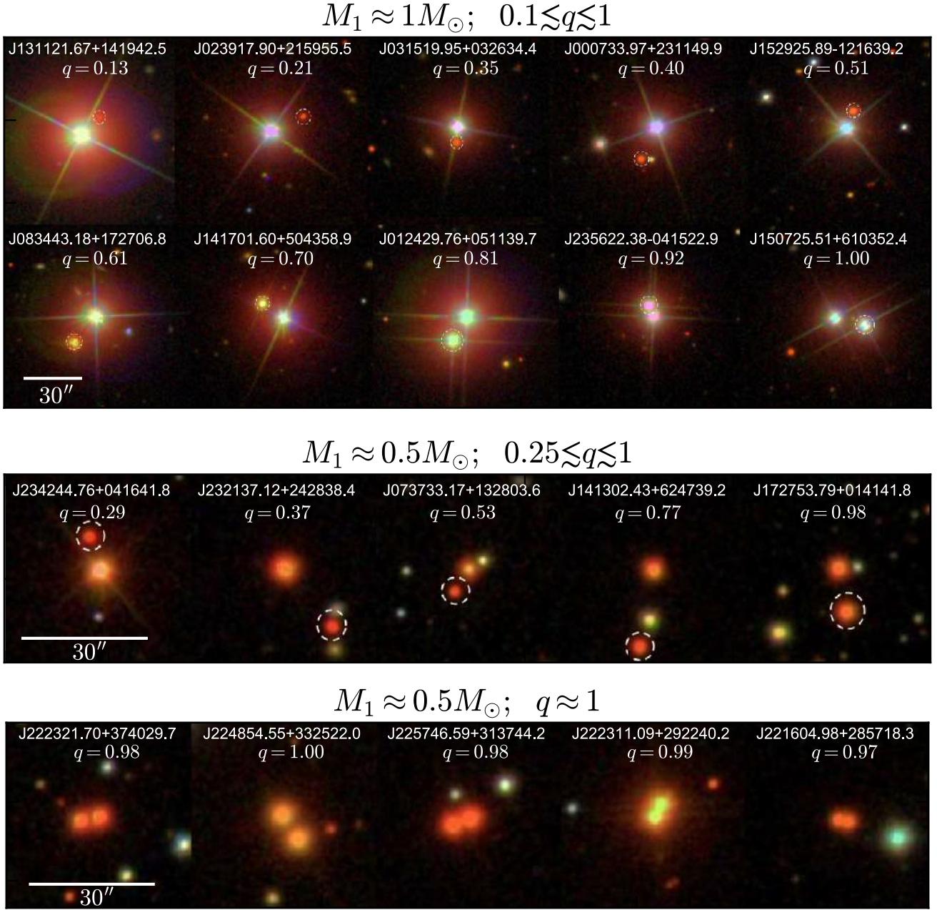
Figure 2. SDSS images of a selection of binaries from our catalogue. Top panel shows binaries in which the primary is a solar-type star ( 0.9 < M_1/M_{\odot} < 1.1 ) and the mass ratio varies from \approx 0.1 to 1. The primary is at the centre of each image, and the secondary is circled. Middle panel shows binaries in which the primary is a late K dwarf ( 0.4 < M_1/M_{\odot} < 0.6 ), again for a range of mass ratios. Bottom panels shows examples of ‘twin’ binaries with near-identical components, each with 0.4 < M_1/M_{\odot} < 0.6 . Each image is 100 (top panel) or 45 (bottom panels) arcsec on a side. Our analysis uses photometry from Gaia , not SDSS. Because the SDSS photometry is ground based, blending and source contamination affect it more severely.
