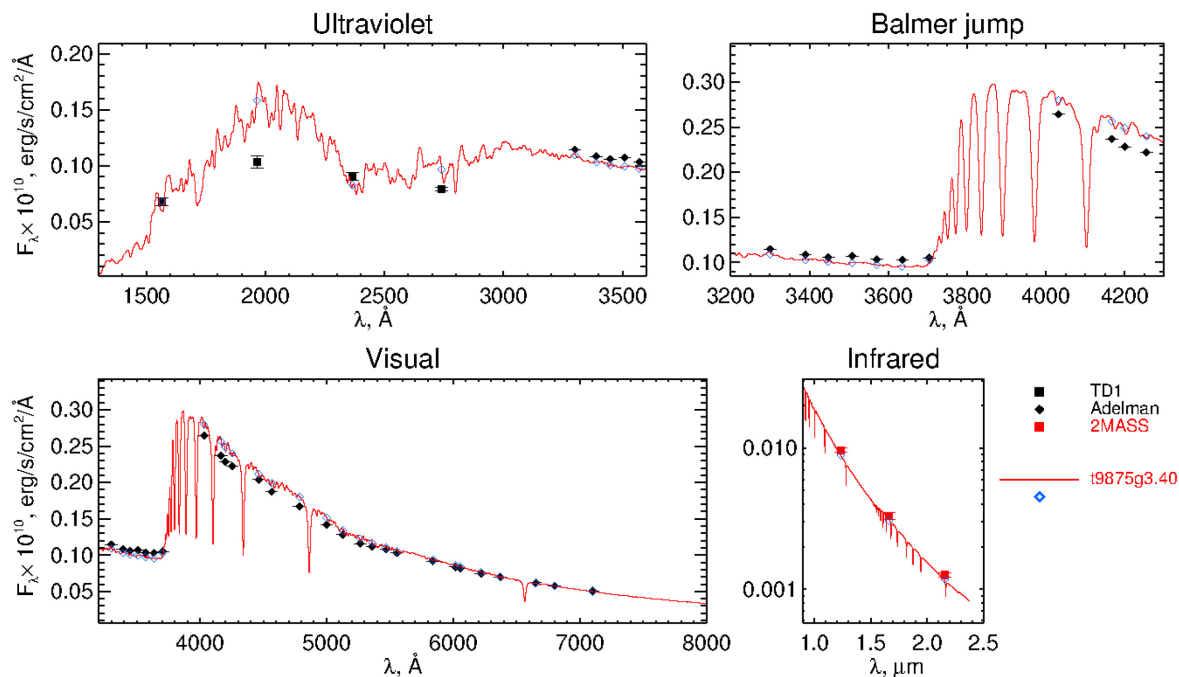
Figure 8. Same as in Fig. 6, but for HD 111133.
