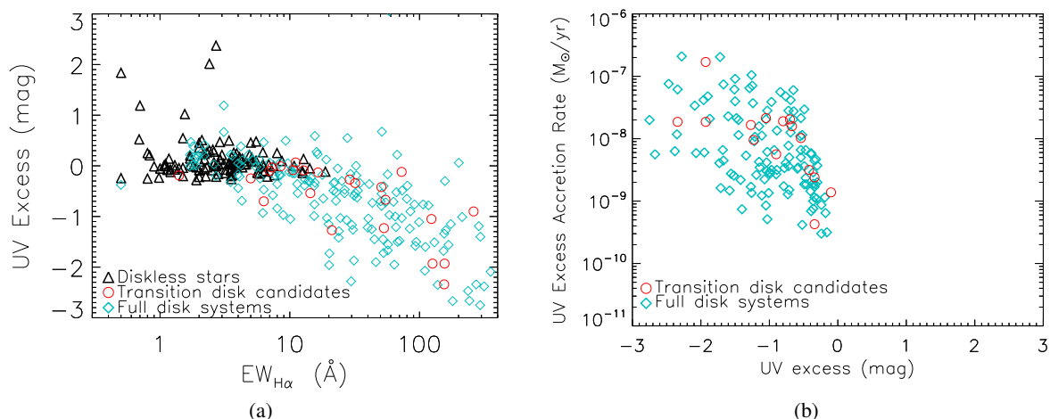
Fig. 10. UV excess as a function of H\alpha equivalent width (a) and mass accretion rate as a function of UV excess (b). More negative values indicate larger UV excess. The UV excess and mass accretion rate were calculated by Venuti et al. (2014) and the H\alpha equivalent width was measured by Sousa et al. (2016) and Dahm & Simon (2005). As expected, diskless stars do not present UV excess, while full disk systems do. Transition disk candidates, in general, present UV excess similar to stars with full disks, which is consistent with active accretion, as discussed in the text.
