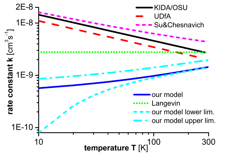
Fig. 2. Temperature dependence of the total rate constant k for the reaction of He + with DME. Solid black line: recommended values from KIDA database according to Eq. (1); dashed red line: recommended values from UDfA according to Eq. (1); dotted green line: Langevin rate constant k_L according to Eq. (4); dashed pink line: classical trajectory scaling according to Eq. (3) (Su & Chesnavich 1982); solid blue line: our calculations; cyan dotted-dashed line: our calculations, upper limit estimate; cyan dashed line: our calculations, lower limit estimate (see text).
