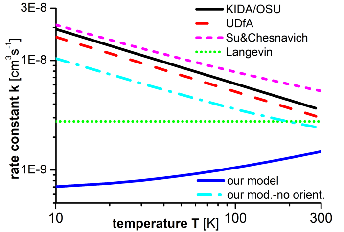
Fig. 3. Temperature dependence of the total rate constant k for the reaction of \text{He}^+ with MF. The curve colours are as in Fig. 2, except for the dashed-dotted cyan line which corresponds to the data calculated using our model and assuming no preferential orientation of the colliding system.
