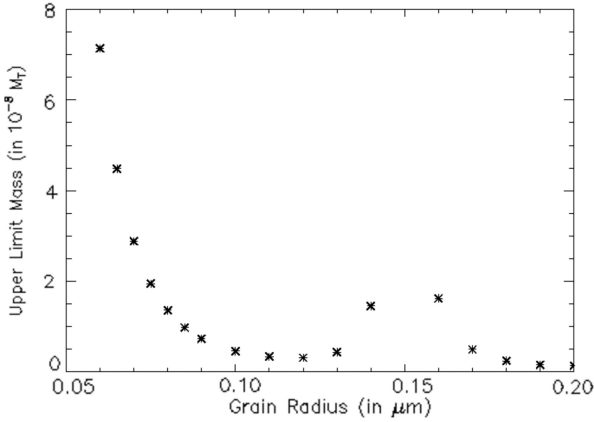
Figure 3. Mass of the disc determined as a function of the grain radius, for an assumed observed polarization of 0.1 per cent. The mass is given in terrestrial mass, ( M_{\oplus} = M_{\oplus} ). Other assumptions are given in the text. There is no symbol for a radius of 0.15 \mu\text{m} due to the very low polarization induced by grains of this size. This leads to a very high disc mass, larger than the scale of this figure.
