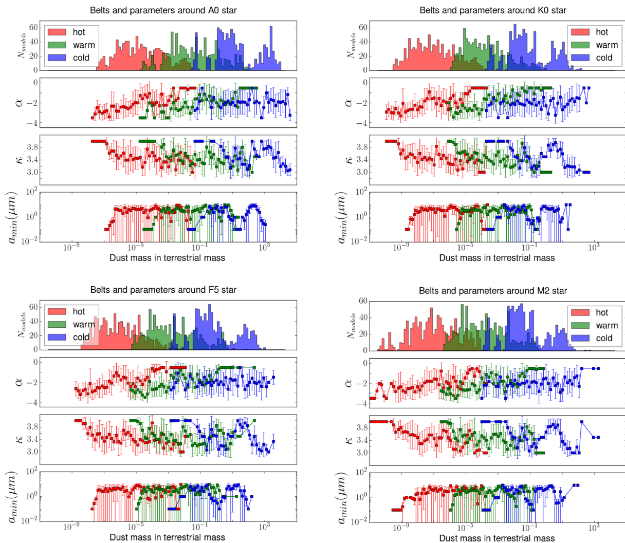
Figure 4. Histograms representing the number of simulations sorted by the mass of the minimum detectable mass of their discs. All 972 disc models are used, including the three stellar positions for simulating eccentricity. Underneath we plot the mean values in each mass bin for the surface density exponent \alpha , the grain-size distribution power-law index \kappa , and the minimum size of the grains, a_{\min} , for the four spectral types and three belts considered (see Table 7). The error bars correspond to 1\sigma and vary according to the number of simulations in each mass bin.
