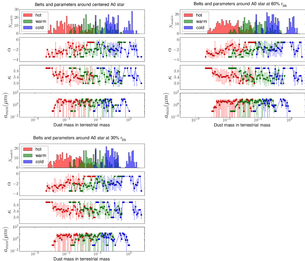
Figure 5. Histograms representing the number of simulations sorted by the mass of the minimum detectable mass of their discs. These histograms present results for only the A0 star and correspond to the top panel of Fig. 4 split into three parts to compare the outcome for each stellar position, centred, at 30 and 60 per cent of r_{\text{in}} . Underneath, we plot the mean values in each mass bin for the surface density exponent \alpha , the grain-size distribution power-law index \kappa , and the minimum size of the grains, a_{\text{min}} , for the three stellar positions and three belts considered. The error bars correspond to 1\sigma and vary according to the number of simulations in each mass bin.
