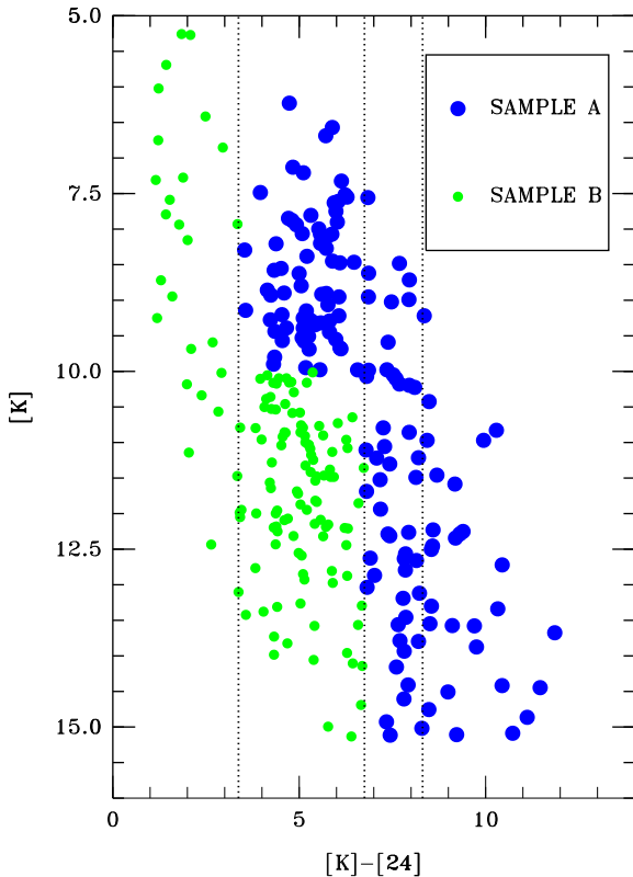
Figure 1. The [K] versus [K] - [24] colour-magnitude diagram of the full sample of Spitzer Young Stellar Object Candidates in Ophiuchus identified by the Cores to Disks Legacy Programme. The vertical lines are the approximate boundaries between Class III, Class II, Flat Spectrum, and Class I objects (left to right). The Spitzer objects were divided into two ODISEA samples. Sample ‘A’, presented in this paper, contains 147 objects, which are Class I and Flat Spectrum sources together with Class II objects brighter than 10 mag in K band.
