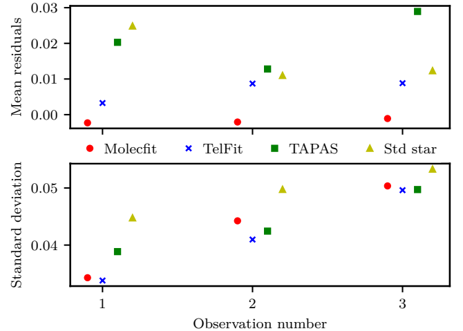
Fig. 5. Mean and standard deviation of the residuals inside the telluric lines for the four telluric correction methods in the wavelength range dominated by H 2 O absorption. The colour code is the same as Fig. 4.
