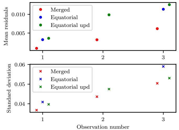
Fig. 13. Mean and standard deviation of the residuals inside the telluric lines. The telluric correction was done with Molecfit using three different atmospheric profiles as inputs. The colour code is the same as Fig. 12.
