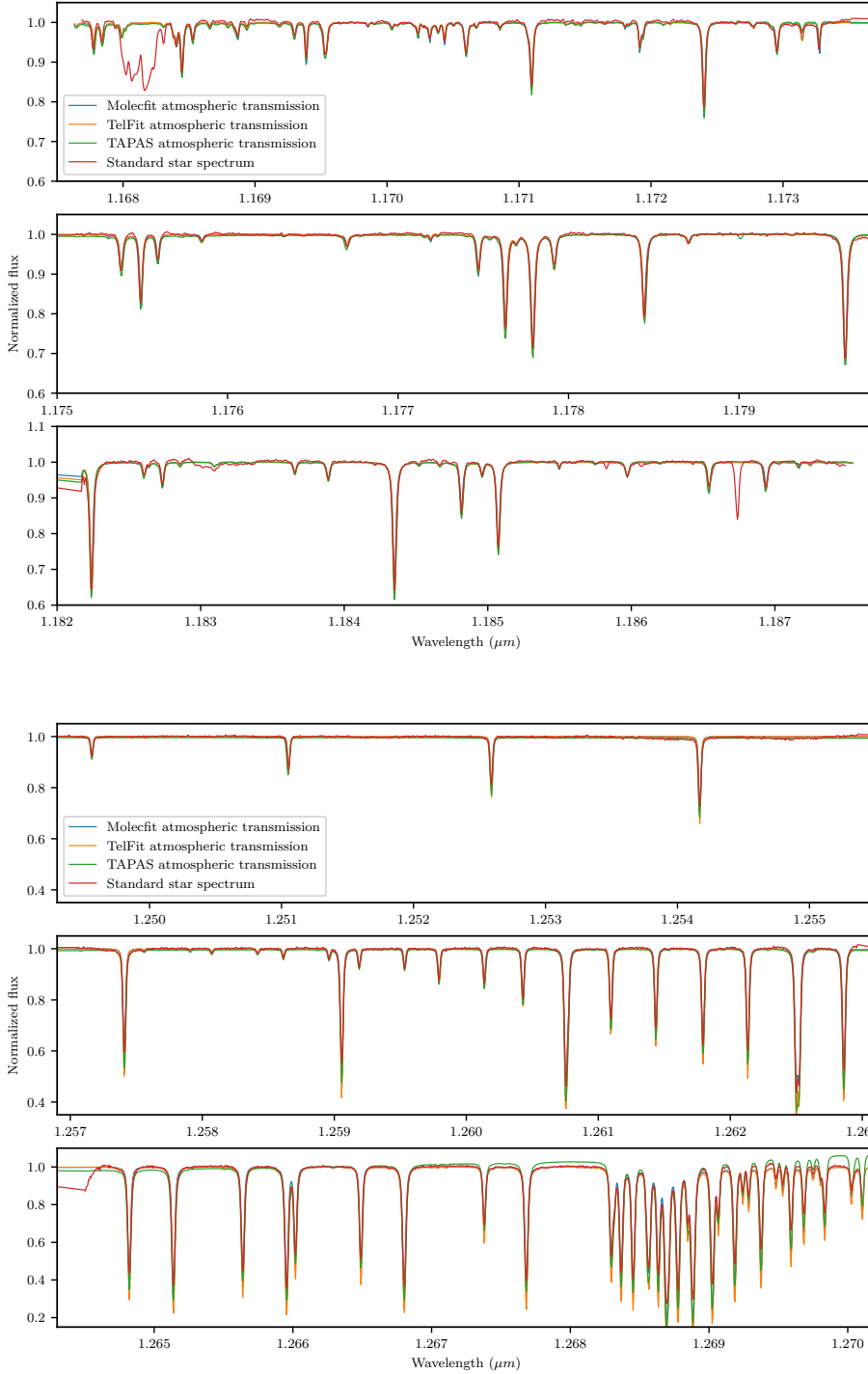
Fig. A.1. Synthetic transmission spectra and the standard star spectrum dominated by water absorption. The blue curve is computed with Molecfit, the orange curve with TelFit, the green curve with TAPAS, and the red curve is the standard star spectrum.
