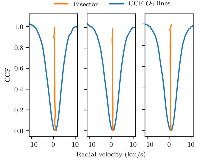
Fig. 8. Cross-correlation function (blue line) and its bisector (orange line) of the O_2 lines from the standard star spectra for observations 4, 5, and 6.
