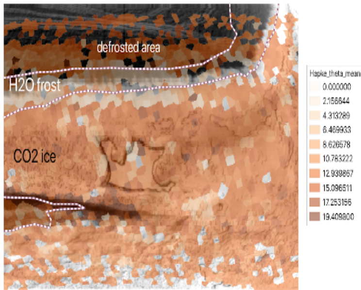
Figure 2: Mars South Pole dataset. Parameter \theta averaged over spectral dimension.
