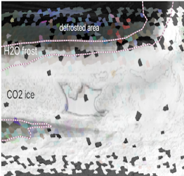
Figure 1: Mars South Pole dataset. Parameter \omega in synthetic colors coding 3 wavelengths.
