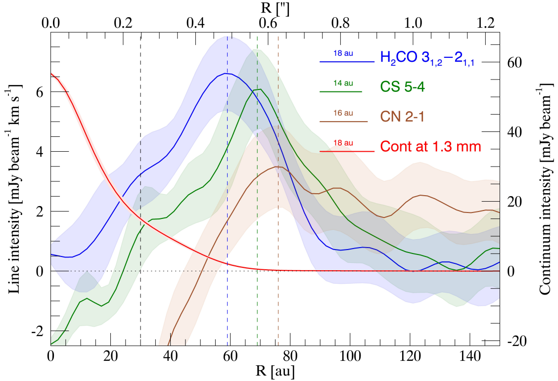
Fig. 2. Azimuthally averaged radial intensity profile of \text{H}_2\text{CO} 3_{1,2}-2_{1,1} (blue), CS 5–4 (green), and CN 2–1 (brown; blending of the three components at 226.87 GHz reported in Table 1) in \text{mJy beam}^{-1} \text{ km s}^{-1} (left axis), and of the 1.3 mm continuum (red) in \text{mJy beam}^{-1} (right axis). The radial distance is indicated in au on the bottom axis and arcseconds on the top axis. The angular resolution of the lines/continuum profiles is indicated by the corresponding horizontal lines. The shaded areas indicate the dispersion of the intensity values around the mean along each annulus in the radial direction. The vertical dashed lines indicate the position of the CO snowline (black), and of the peaks of the emission in \text{H}_2\text{CO} 3_{1,2}-2_{1,1} (blue), CS 5–4 (green), and CN 2–1 (brown).
