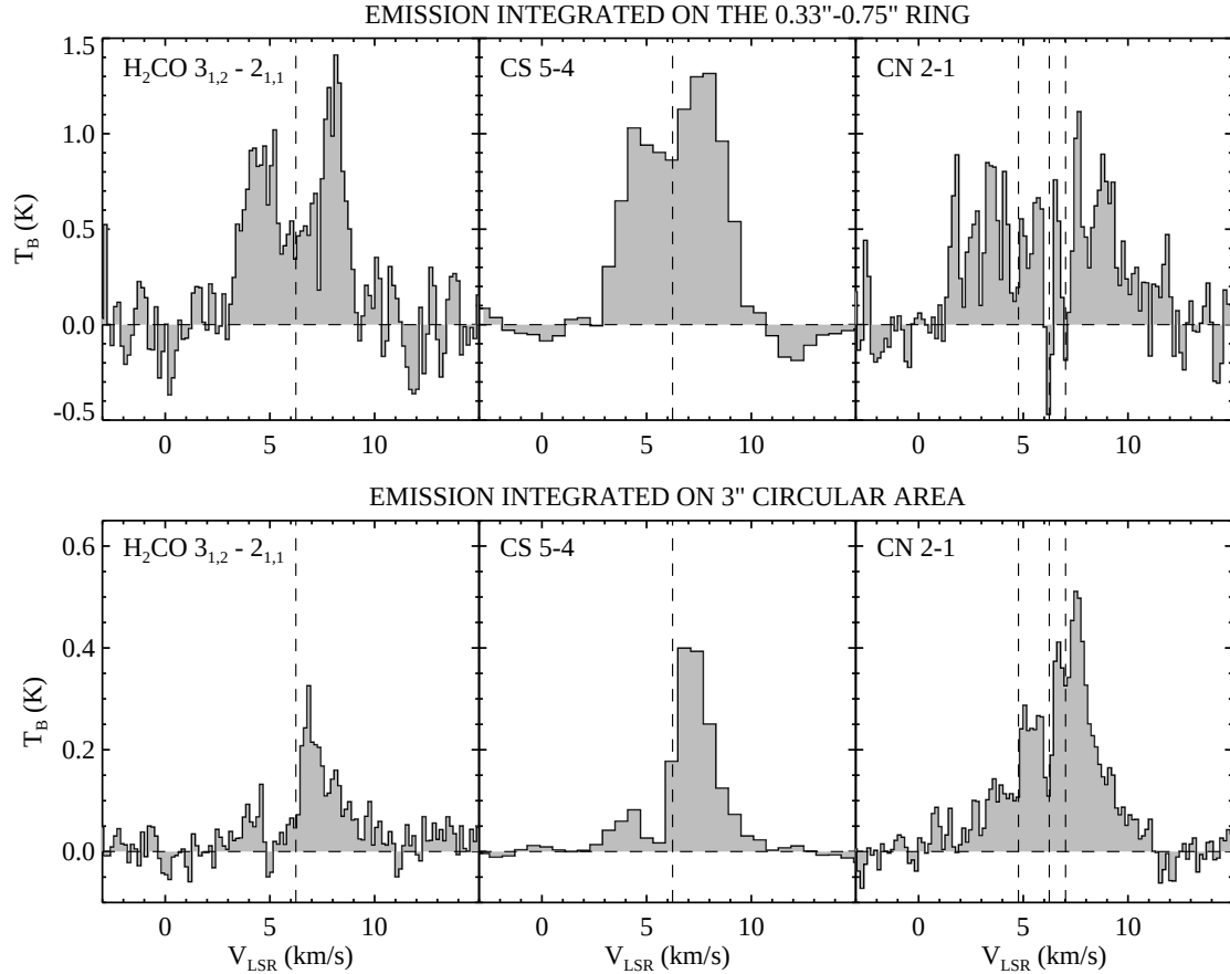
Fig. B.1. \text{H}_2\text{CO } 3_{1,2}-2_{1,1} , CS 5-4, and CN 2-1 spectra integrated over a 0''.33-0''.75 ring area ( top panels ) and over a 3'' circular area ( bottom panels ), in brightness temperature T_B . The vertical dashed lines indicate the systemic velocity, V_{\text{sys}} = +6.24 \text{ km s}^{-1} . For CN 2-1 the velocity scale corresponds to the brightest of the three hyperfine components at 226.87 GHz reported in Table 1 ( N=2-1 , J=5/2-3/2 , F=7/2-3/2 ), and the position of the two fainter components is indicated by the vertical dashed lines.
