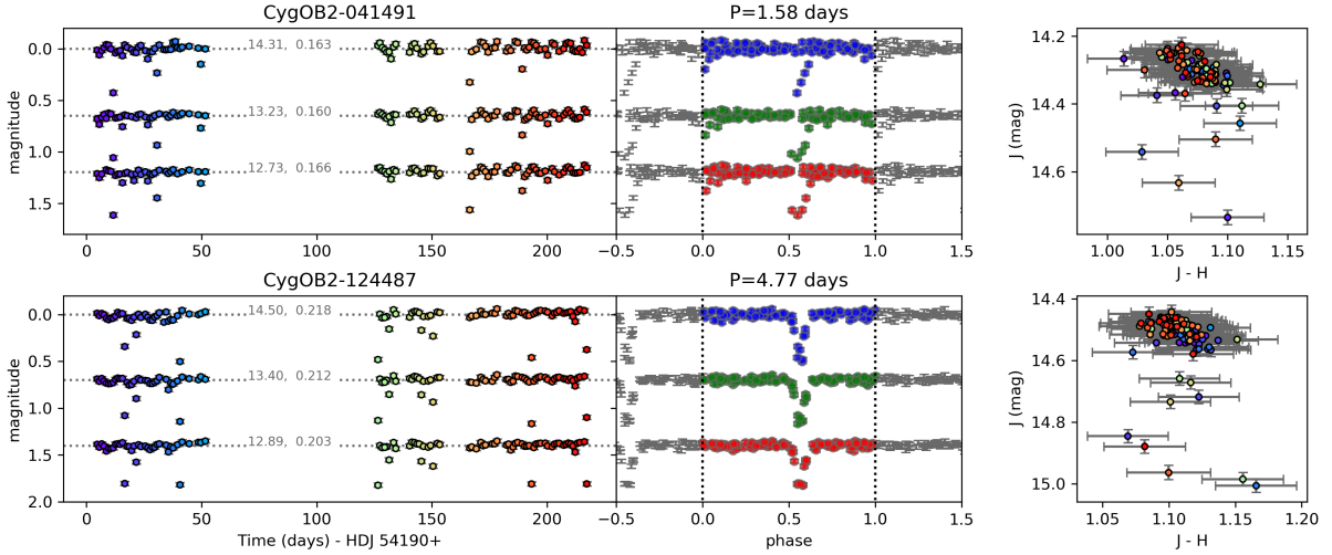
Fig. 16. Two multiperiodic eclipsing binary candidates. Left: J , H , and K light curves for each star. The median magnitude and ptp amplitude are written in the plot, and the colors reflect the date of the observation, as in Fig. 4. Middle: phased light curve for each band, folded using the detected period attributed to the occultation feature. J , H , and K bands are shown as blue, green, and red respectively. Figure 17 shows the folded light curves for the secondary period. Right: J vs. J-H CMD. Colors reflect the date of the observation, as in Fig. 4.
