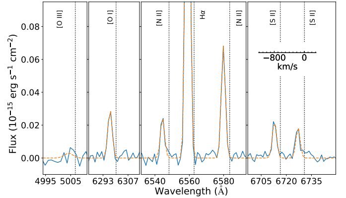
Fig. 4. Selected spectral regions extracted at the knot. The axis scaling is similar in all panels in velocity and flux, i.e., the velocity scale shown in the [S\text{ II}] panel applies to all four panels equally.
