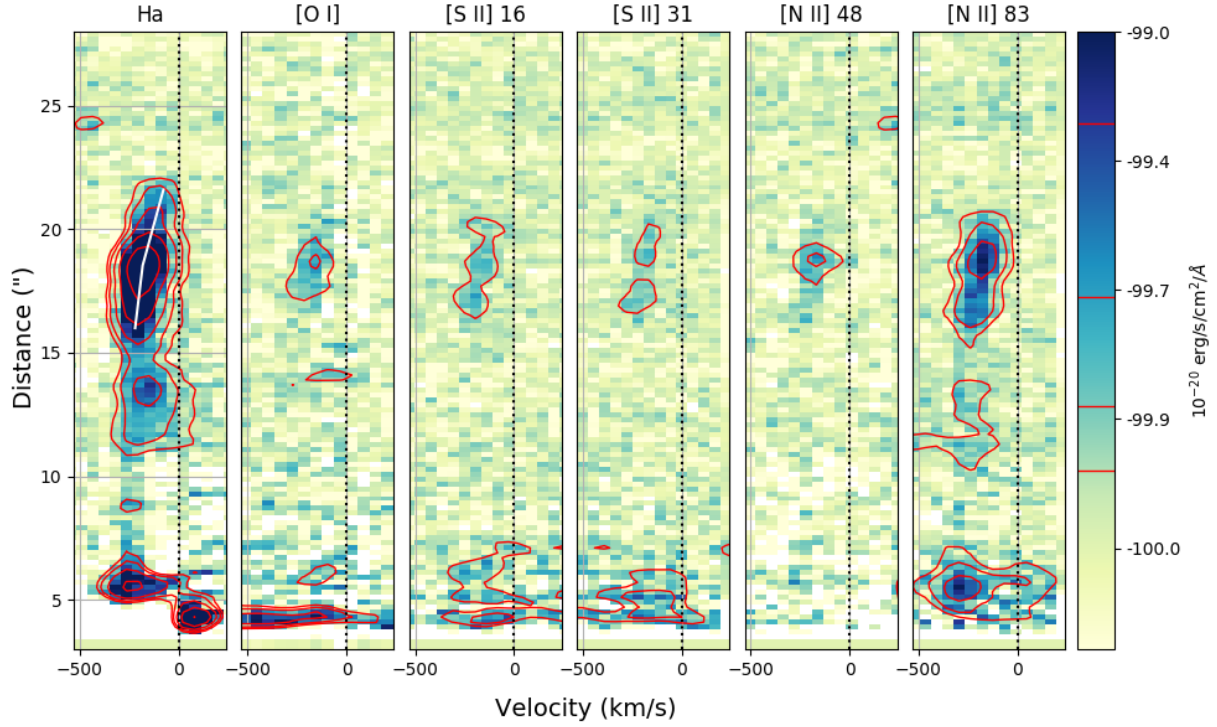
Fig. 3. Position-velocity diagrams of the main jet emission lines. From left to right: H\alpha , [O\text{ I}] \lambda 6300 , [S\text{ II}] \lambda 6716 , [S\text{ II}] \lambda 6731 , [N\text{ II}] \lambda 6548 , and [N\text{ II}] \lambda 6583 . The white line in the H\alpha panel indicates the peak velocity.
