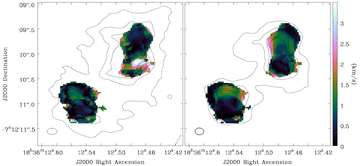
Fig. 14. Velocity dispersion difference (from second moment maps) at each pixel in G24 between ( left ) \text{H}_2\text{CO} (3) and \text{NH}_2\text{CHO} (2) and ( right ) \text{HNCO} (1) and \text{NH}_2\text{CHO} (2). The contours show the integrated intensity maps for \text{H}_2\text{CO} (3) and \text{HNCO} (1) as in Fig. 5. The velocity scale is the same for both panels.
