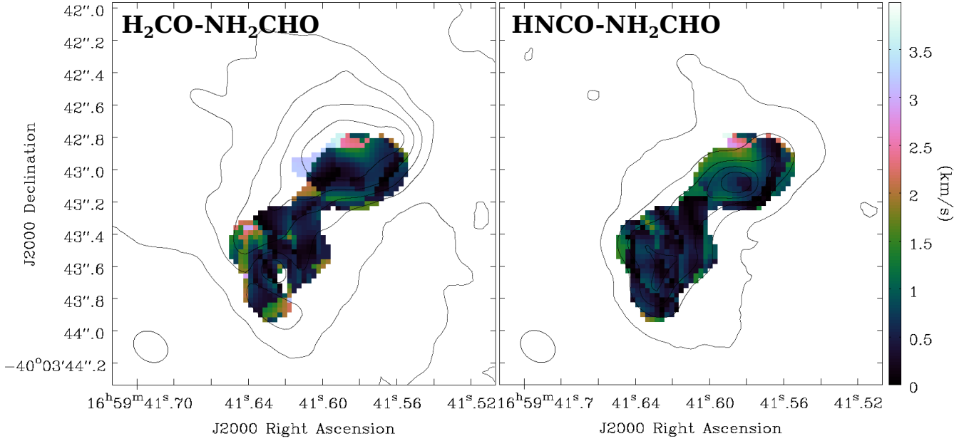
Fig. 11. Velocity difference (from first moment maps) at each pixel in G345 between ( left ) H 2 CO (2) and NH 2 CHO (1) and ( right ) HNCO (2) and NH 2 CHO (1). The contours show the integrated intensity maps for H 2 CO (2) and HNCO (2) as in Fig. 6. The velocity scale is the same for both panels.
