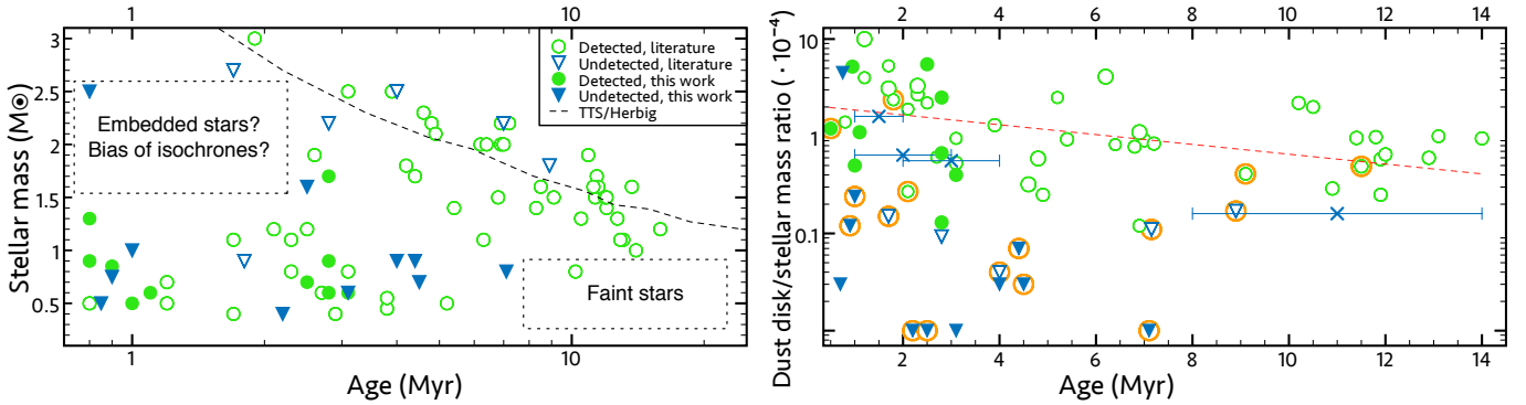
Fig. 6. Stellar and disk mass with time. Left panel: stellar mass for the sample of this work compared with the literature sample analyzed by Garufi et al. (2018). The dashed line is the formal threshold of G0-type stars. Right panel: same as the left panel for the dust disk mass normalized to the stellar mass. The blue crosses indicate the median ages for the Taurus, Lupus, Chamaleon, and Upper Sco regions. The orange circles denote the presence of a visual companion at a few dozen au from that target. The dashed line is the fit to the disks that were available before this work.
