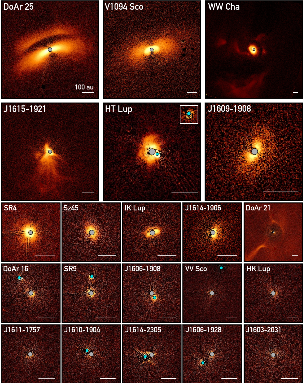
Fig. 1. Overview of the sample. For each target, the Q_0 image in the H band is shown. First two rows: host disks with clearly visible substructures, the third row: contains disks with no or marginal evidence of substructures, and the last two rows: non-detections. The horizontal bars indicate a physical scale of 100 au. The main star is behind the gray circle in the center, symbolizing the coronagraph. Stellar companions are indicated by cyan circles. Each image has a different logarithmic color scale, chosen to highlight all relevant features. The C component of HT Lup is shown in the inset image, although the star would lie outside of the box. North is up, and east is left.
