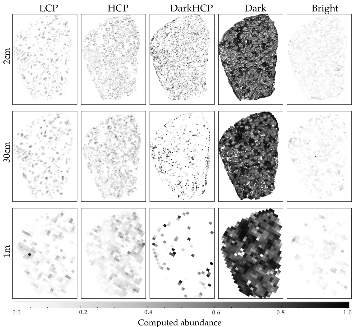
Fig. 5. The linear unmixing results using FCLSU for the five spectral endmembers selected using the supervised method.
