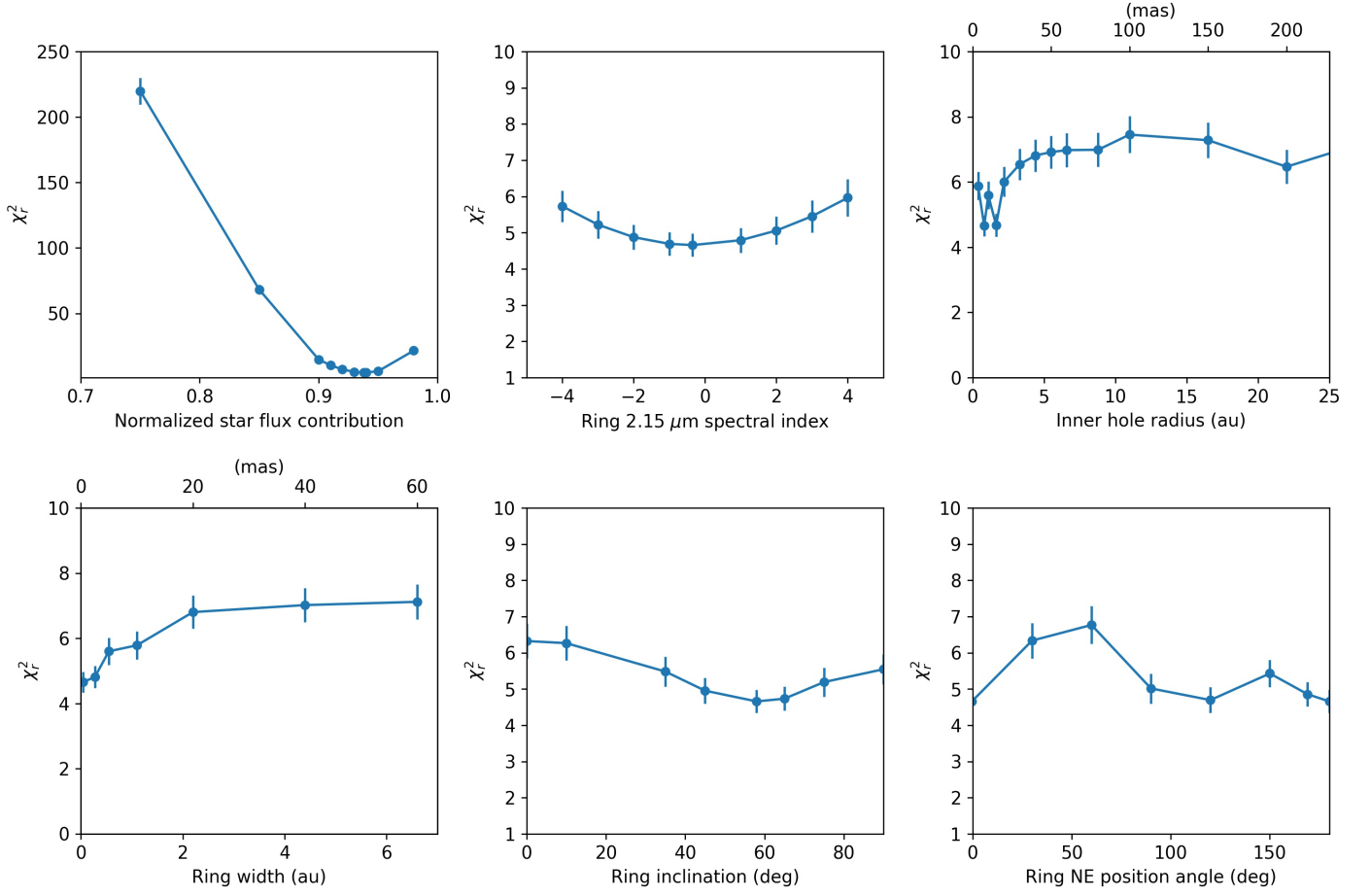
Fig. B.2. Reduced chi-squared \chi_r^2 from the geometrically thin ring model squared visibility fit as a function of the different model parameters. Each point represents a squared visibility fit with the respective parameter fixed to that value while the other parameters are set free.
