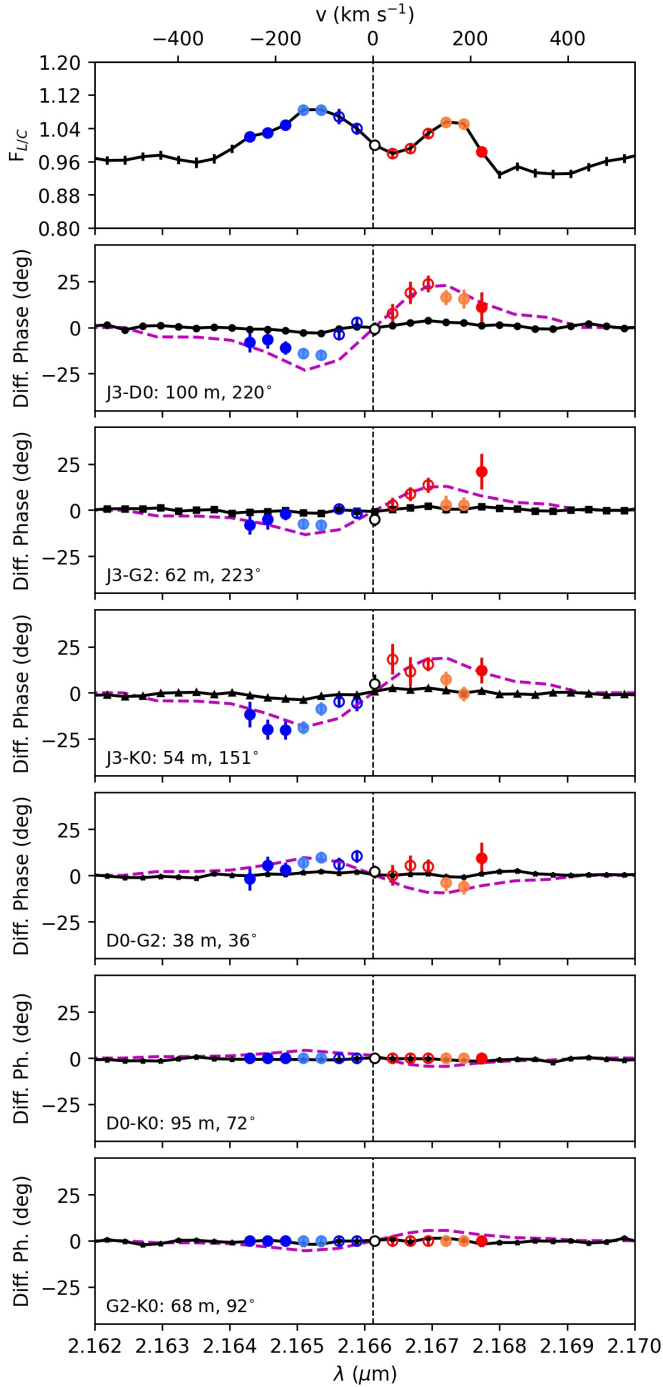
Fig. 4. HD 141569 spectrum ( top ), total (black circles and line), and pure-line differential phases (colored signs) along the different base-lines. D0-K0 and G2-K0 baseline pure-line differential phases are set to zero. The colors refer to the different spectral channels. Dashed magenta lines represent the pure-line differential phases of the analytical Keplerian disk model described in Sect. 5.3.
