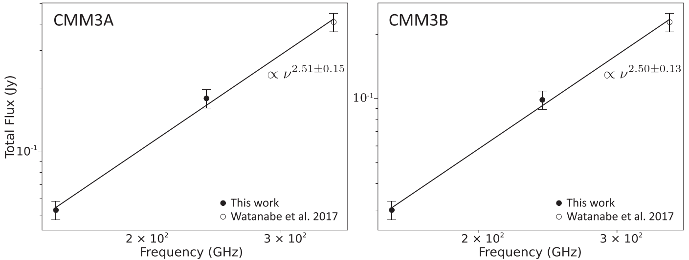
Figure 4. The spectral index derived from the total flux. The closed circles represent the results of this work, while the open circle represents the 0.8 mm data taken from Watanabe et al. (2017). The horizontal axis shows the frequency of the continuum images and the longitudinal axis shows the total flux. Errors are 10% of each total flux. The flux is measured for a 0''.6 \times 0''.6 area for CMM3A and CMM3B.
